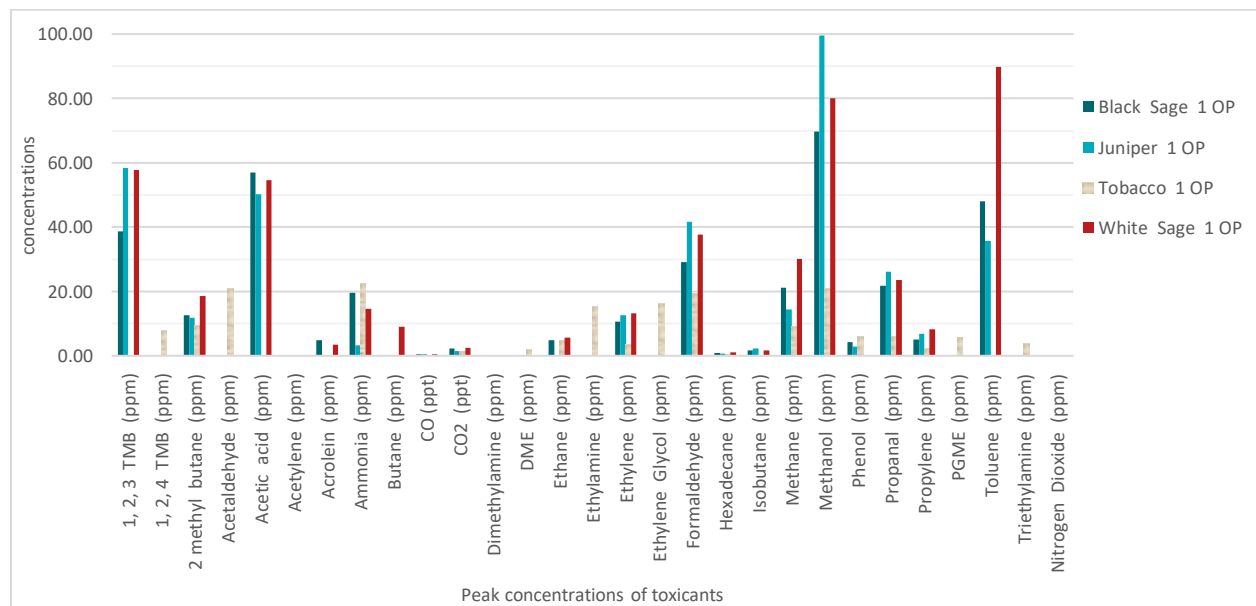
Figure 5. Peak concentrations of toxicants produced from the four samples during oxidative pyrolysis (OP) in tube furnace
