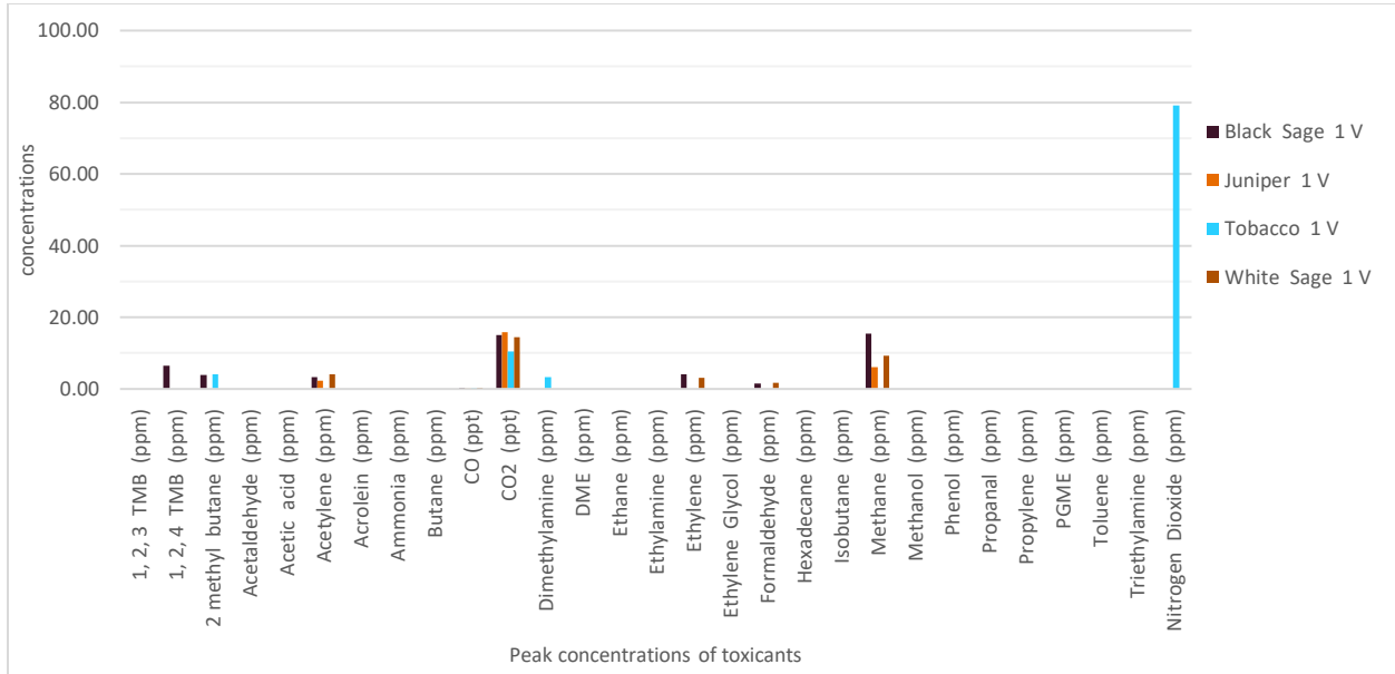
Figure 6. Peak concentrations of toxicants produced from the four samples during vitiated (V) thermal decomposition in tube furnace
