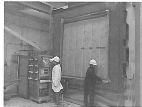
IRC researchers prepare a full-scale wall specimen for an experiment in the Envelop Environmental Exposure Facility
