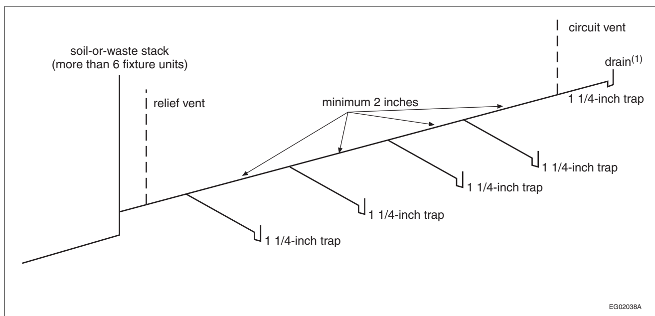
Figure A-2.5.3.1.-K
