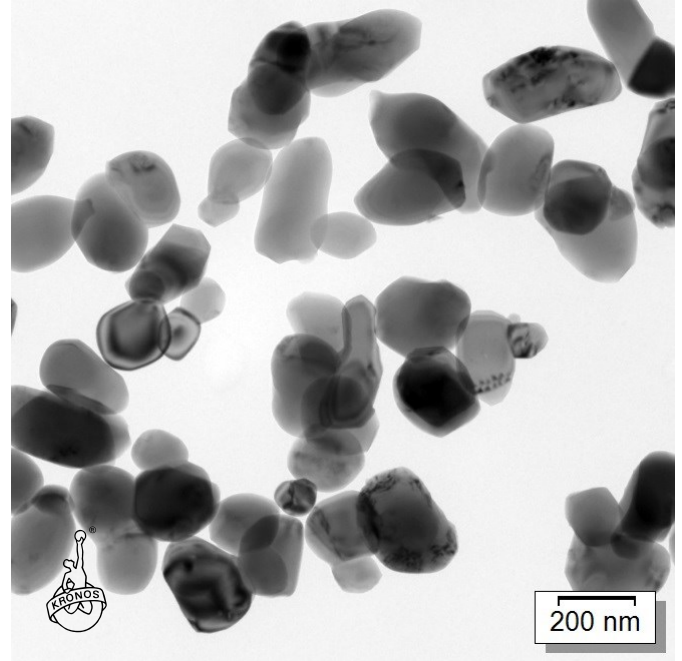
Figure 2: K2971 – TEM-Image
