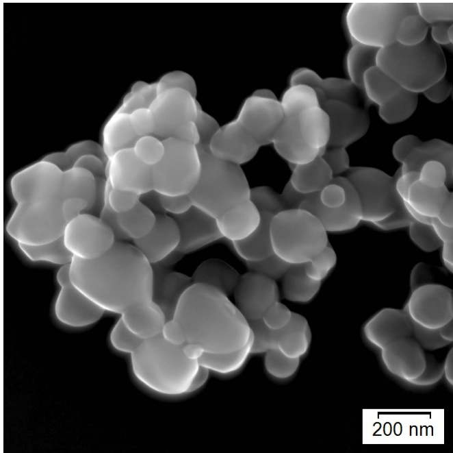
Figure 3: K1171 – SEM-Image
