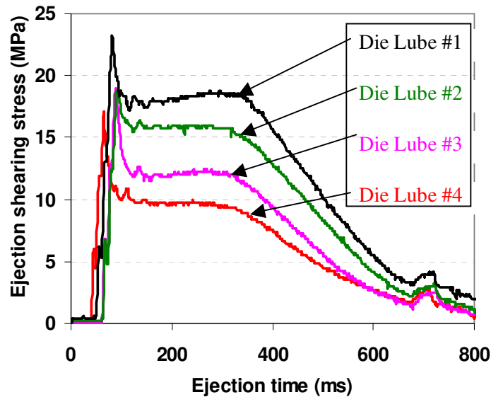
Figure 5: Effect of DWL lubricants (“Die Lubes” #1 to #4) on the ejection performance of Mix 2 (gears #2) compacted at a fixed density.
