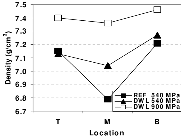
Figure 10: Axial density variation of gears #2 pressed at different compacting pressures with and without die wall lubrication technique.
