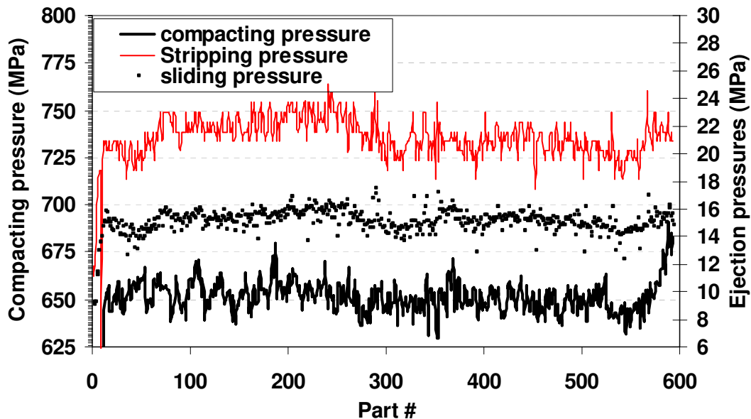
Figure 11: Part-to-part compacting pressure and ejection stability of half inch thick Izod bars pressed with Mix 1 at a density of 7.20 \text{ g/cm}^3 .
