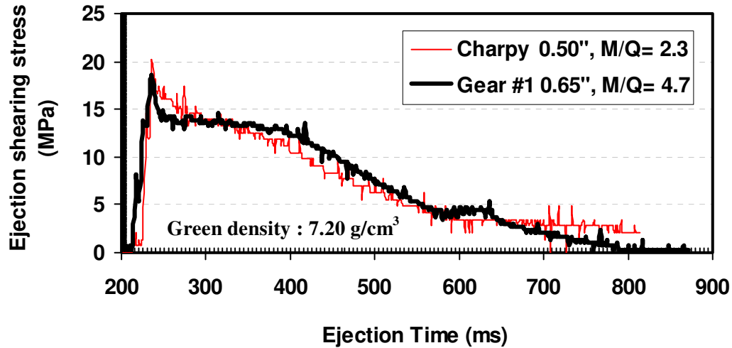
Figure 7: Effect of aspect ratio on the ejection performance of Mix 1 compacted with DWL. When compacting complex parts at high pressures such as gear G#2 having a high aspect ratio ( M/Q = 13.8 ), the benefits of using die wall lubrication vs. conventional pressing are significant, both in terms of green density (Figure 8) and ejection performance (Figure 9). The higher densification observed with Mix 2 can be explained both by the excellent lubrication at die walls and by the lower amount of internal lubricant, that postpone the occurrence of inhibition of compaction at high pressures due to the volume of lubricant entrapped in the porosity.
