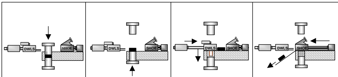
Figure 13: DWL system configuration where the spraying unit actuator is independent of the feed shoe.
