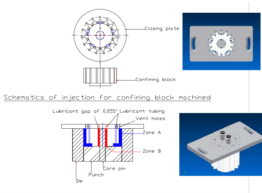
Figure 4: Drawing of the spraying unit (confining block and closing plate) used to apply lubricant both on die walls and core pin when processing gears #1.
