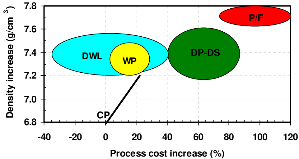
Figure 1: Cost to performance ratio as respect to conventional pressing of regular mixes [1].
