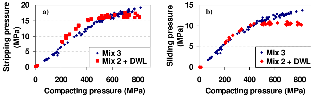
Figure 9: Ejection performance of Mix 2 compacted with DWL vs. the reference mix, Mix 3 (conventional pressing): a) stripping pressure, b) sliding pressure
