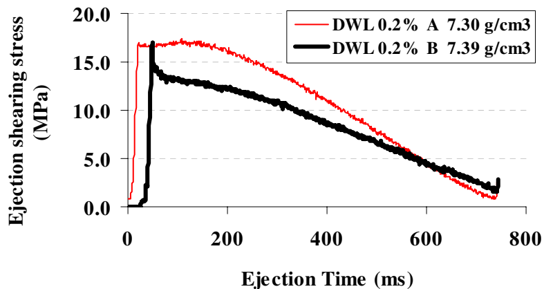
Figure 6: Ejection curves of Mix 2 compacted with two different admixed lubricants (0.2% lubricant A or 0.2% lubricant B). Compacting pressure was 827 MPa (60 tsi) and die wall lubricant was Die Lube #2.
