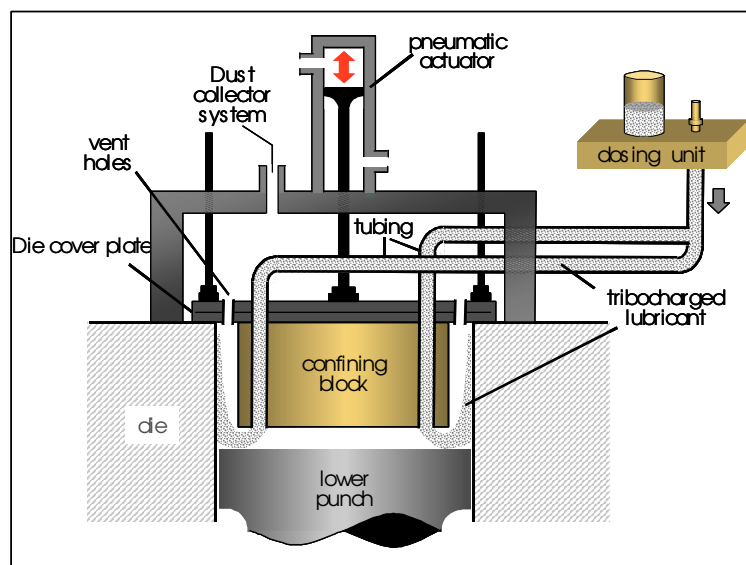
Figure 2: Schematic diagram of the die wall lubrication system.
