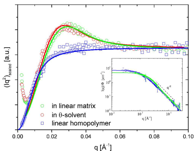
Figure 5. Comparison of the experimental ring form factor in \theta -solvent and in a comparable linear matrix. Intensities were normalized to the same concentrations and rescaled at high scattering vectors. Symbols are explained in the figure legend. Solid lines are best fit curves to the ideal Gaussian ring form factor. A small difference in the radius of gyration, i.e., 72 to 76 Å, can be noticed from the peak positions. For further comparison also the form factor of the linear matrix chain which is a perfect random walk Debye chain is included. The inset shows the direct intensity comparison ( I vs q ) for latter ideal linear chain blend and the ring-linear blend.
