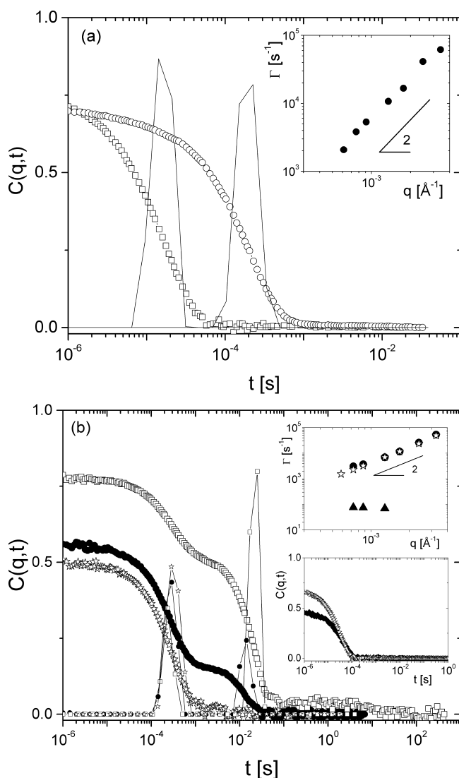
Figure 4. (a) Intermediate light scattering function for a ring PS R161 solution in d_8 -toluene (0.5 wt %) at 33 °C. Data are shown for the lowest and highest scattering angles, 30° (circles) and 150° (squares). The respective distributions of relaxation times obtained from CONTIN analysis are also shown. Inset: the q -dependence of the extracted characteristic relaxation rate. (b) Intermediate light scattering function for the same R161 solution in d_{12} -cyclohexane (0.012 wt %) and different temperatures and scattering angles, indicated in the plot: 33 °C and 30° (open squares); 40 °C and 30° (bold circles); 50 °C and 30° (open stars). The respective distributions of relaxation times obtained from CONTIN analysis are also shown. Insets: (top) Respective q -dependent characteristic relaxation rates at 40 and 50 °C. The slow mode 40 °C is depicted by bold triangles. (bottom) Intermediate light scattering function for a linear PS (250 000 g/mol) solution in d_8 -toluene (0.024 wt %) at a scattering angle of 150° and two temperatures, 25 °C (bold symbols) and 50 °C (open symbols).
