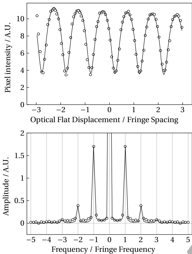
Figure 3. Above: Interferogram recorded at a single image pixel while moving the optical reference flat through 3 wavelengths of the 544 nm laser. Solid line shows a fit to a Fizeau fringe as described in the text. Below: Corresponding Fourier amplitude spectra.
