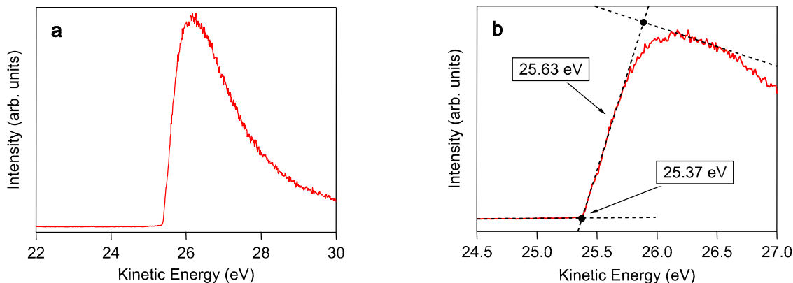
Figure S4. a) Secondary electron energy distribution curve (SEEDC) from a solution of 2 wt% FeOOH nanoparticles dispersed in water under an applied bias of -25 V. b) Extrapolation of the cut-off energy which is found at 25.63( \pm 0.08) eV.
