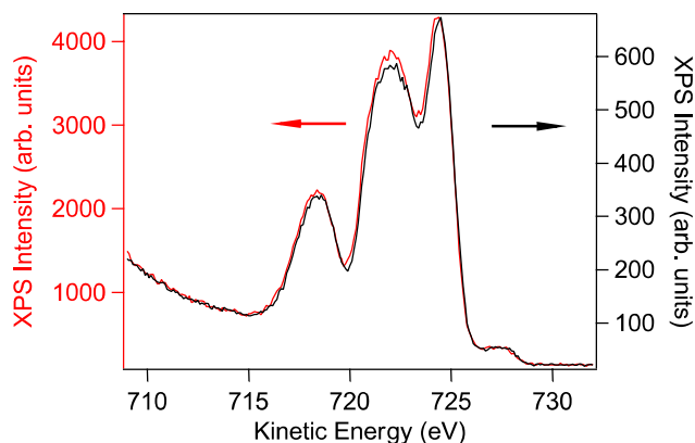
Figure S3. On-resonance valence band spectra for a solution of 2 wt% FeOOH nanoparticles dispersed in water measured with different photon fluxes. The optimized photon flux was reduced by closing the beamline exit slits
