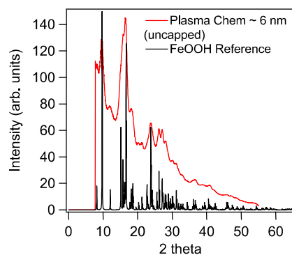
Figure S1. X-ray diffraction measurement of the iron oxide nanoparticles purchased from PlasmaChem (red line) compared to the XRD reference for goethite (FeOOH).
