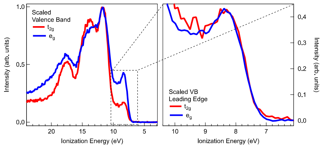
Figure S6. Left side: RPES spectra across the Fe L_3 absorption edge at the t_{2g} (red) and e_g (blue) resonances taken in a dispersion with a substantially higher concentration of FeOOH NPs in the probed volume (caused by a surfactant that encapsulates the NPs and makes them more hydrophobic) that ensured sufficient spectral intensity for the comparison. The two spectra have been normalized to the peak intensity of the highest resonance for comparison. On the right side a close-up view of the VB leading edge, normalized to the peak intensity of the first participant resonance of both spectra is shown. Both spectra evidence the same position of the VBM edge which is resonantly enhanced by participant decay. The position of
