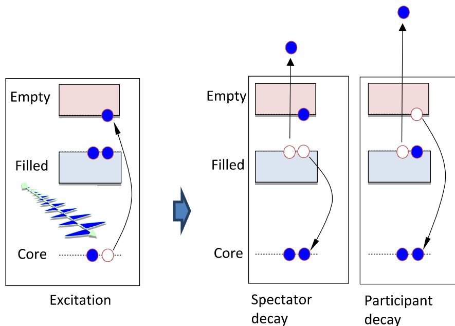
Figure S5. Schematic energy level diagram in Resonant photoemission. a) schematics of core electron excitation to empty state, followed by b) decay of the core hole in which the excited electron spectates the emission of Auger electron and c) core hole decay in which the excited electron participates in de-excitation and Auger electron emission. The Auger electron kinetic energy of c is lower (inelastic) than that of b (elastic).
