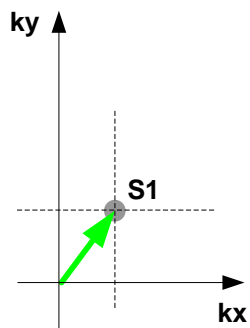
b) Excitation
