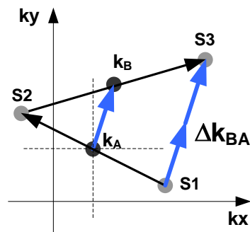
d) Translation
