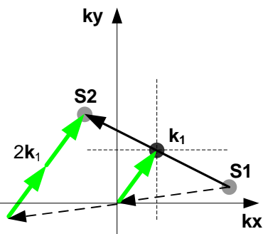
c) Refocusing
