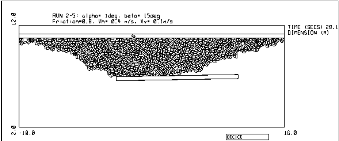
Figure B-49: Snapshot of Run 2-5 at t= 28.19 s
