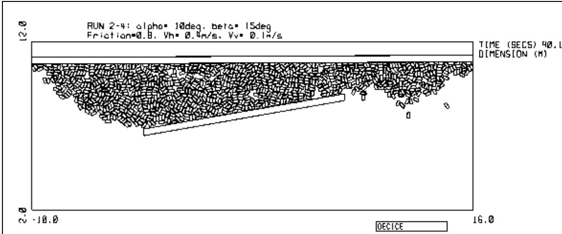
Figure B-43: Snapshot of Run 2-4 at t= 40.19 s
