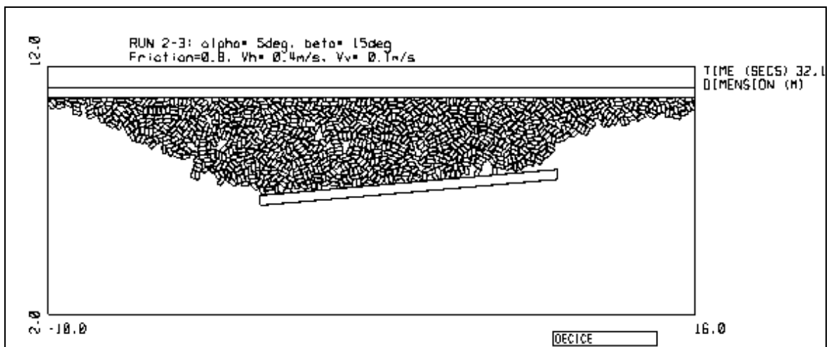
Figure B-27: Snapshot of Run 2-3 at t= 32.19 s
