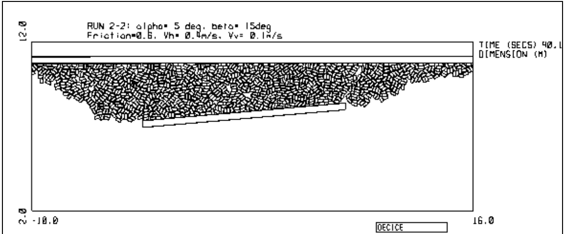
Figure B-19: Snapshot of Run 2-2 at t= 40.19 s
