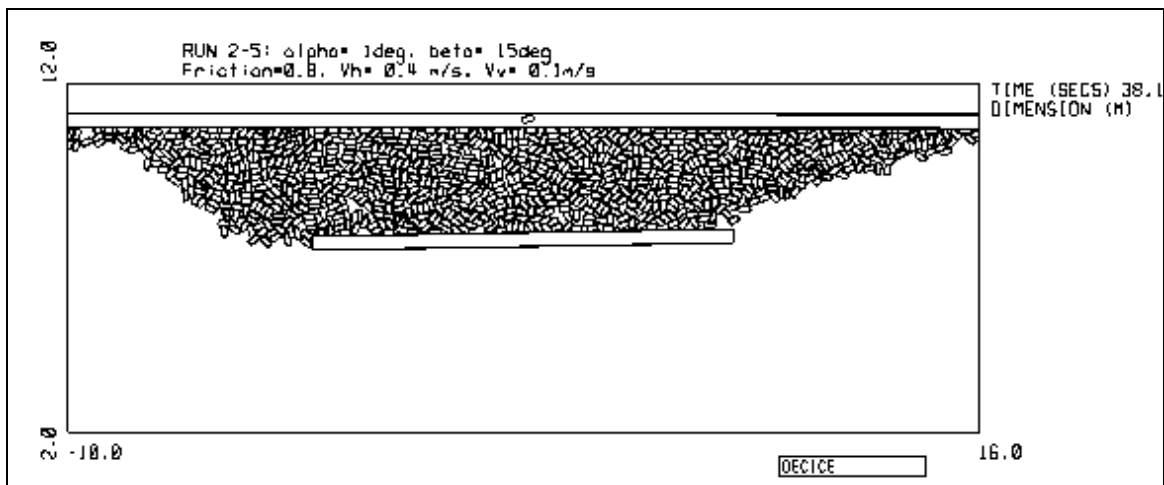
Figure B-54: Snapshot of Run 2-5 at t= 38.19 s
