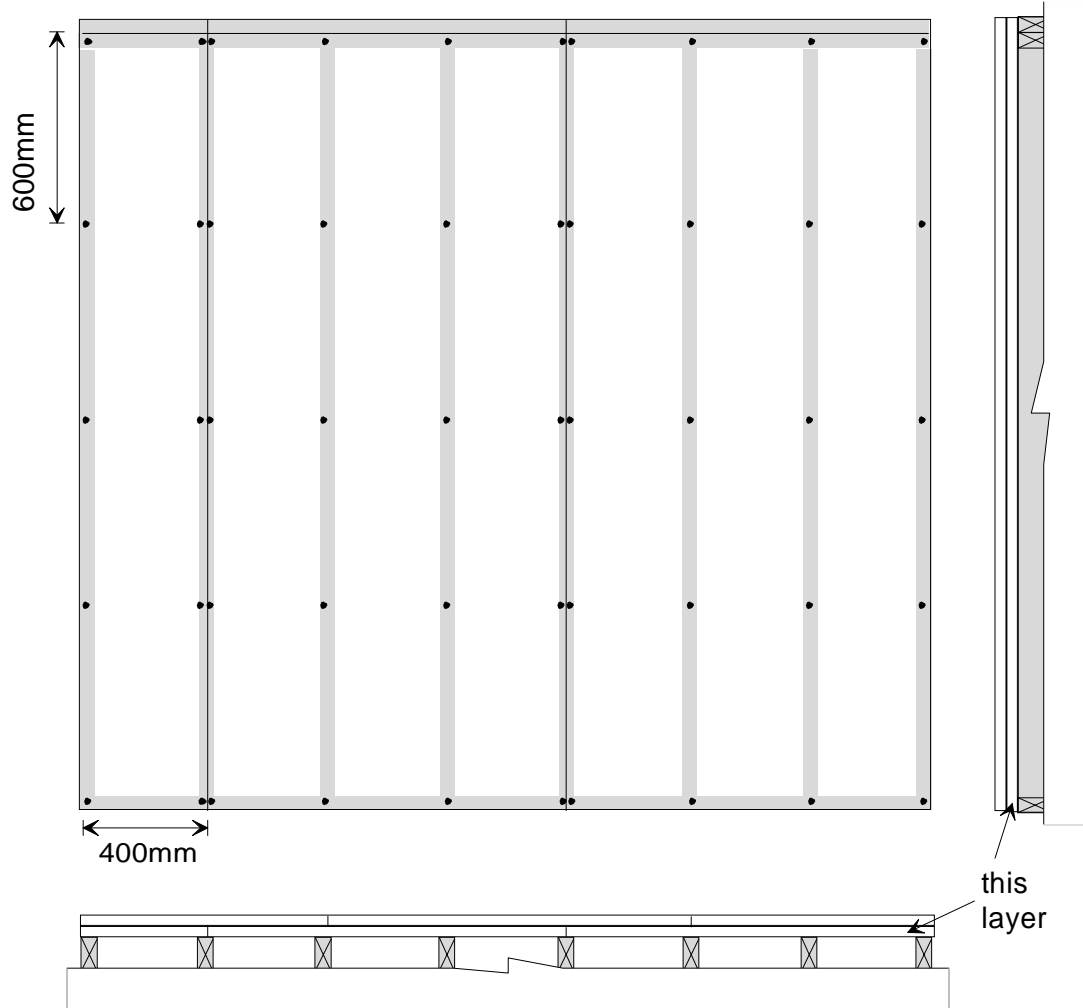
Figure A-5: Base-ply of two-ply gypsum board attached parallel to wood studs at 400 mm o.c., double plate at top, single plate at bottom. Meets requirements of CAN/CSA-A82.31-M91, Clause 7.3.4. Drawing not to scale.
