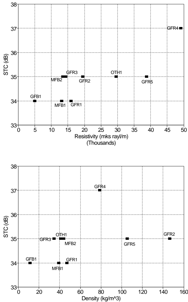
Figs. 3(a) and 3(b): Sound transmission class (STC) versus density and airflow resistance of the materials. Specimens are coded as follows: GFB is glass fibre batt, GFR is glass fibre rigid board, MFB is mineral fibre batt.
