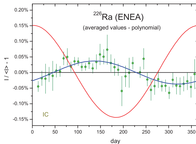
Figure 9. Annual average residuals from exponential decay for ^{226}\text{Ra} activity measurements with the ENEA IC, in which the input data were first detrended by means of the trend line in figure 8.
