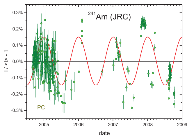
Figure 44. Residuals from exponential decay for ^{241}\text{Am} activity measurements with a proportional counter at JRC.
