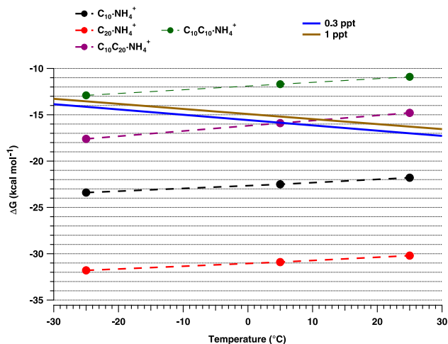
Figure 8. Quantum chemical calculations of Gibbs free energies for cluster formation at -25 , 5 and 25^\circ\text{C} . Solid lines represent the required \Delta G for equilibrium between evaporation and collision rates at 0.3 and 1 \text{ pptv} of the HOM mixing ratio, respectively. Markers show the \Delta G for each cluster (organic core clustered with \text{NH}_4^+ ) at the three temperatures. \text{C}_{10} \cdot \text{NH}_4^+ (black circles) represent the monomer, \text{C}_{20} \cdot \text{NH}_4^+ (red circles) represent the covalently bound dimer, \text{C}_{10}\text{C}_{10} \cdot \text{NH}_4^+ (green circles) represent the dimer formed by the clustering of two monomers and \text{C}_{10}\text{C}_{20} \cdot \text{NH}_4^+ (purple circles) denote the preferential pathway for the trimer cluster (see Table 3).
