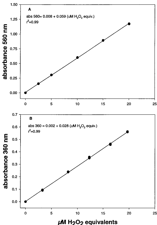
Figure 1. Standard curves relating \mu\text{M H}_2\text{O}_2 equiv (X) to (A) absorbance units at 560 nm (Y) as determined by the FOX assay or (B) absorbance units at 360 nm (Y) as determined by the iodometric assay.
