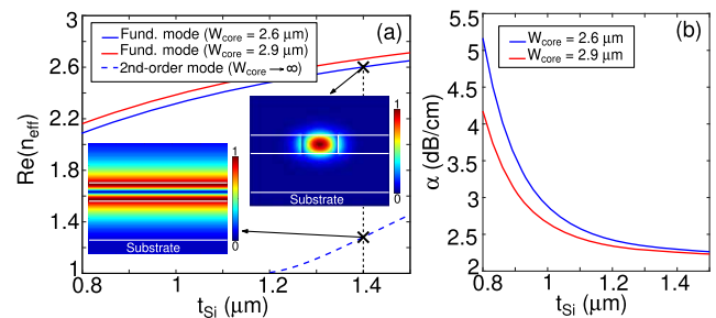
Fig. 2. (a) Real part of the effective indices ( n_{\text{eff}} ) versus the Si thickness ( t_{\text{Si}} ) for the fundamental mode ( W_{\text{core}} = 2.6 \mu\text{m} ) and the second-order vertical mode ( W_{\text{core}} \rightarrow \infty ) supported by the suspended waveguides. Simulation data: t_{\text{BOX}} = 3 \mu\text{m} , n_{\text{SWG}} = 1.72 . The real part of the effective index of the final designed waveguide with W_{\text{core}} = 2.9 \mu\text{m} is also included. Insets: transverse field distributions for the first two modes ( W_{\text{core}} = 2.6 \mu\text{m} , W_{\text{core}} \rightarrow \infty ) when t_{\text{Si}} = 1.4 \mu\text{m} . (b) Power loss of the fundamental vertical mode of the suspended waveguide with W_{\text{core}} = 2.6 \mu\text{m} and the finally designed waveguide as a function of the waveguide silicon thickness t_{\text{Si}} .
