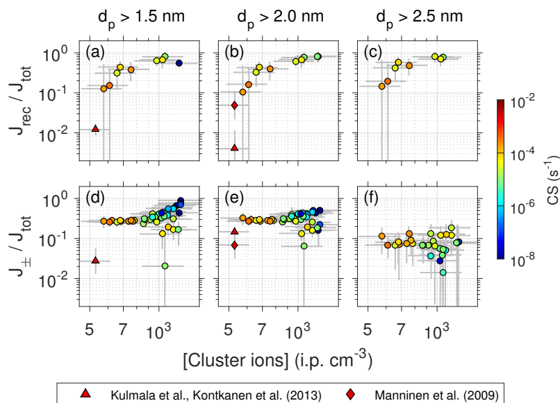
Figure 9. Comparison of CLOUD (system IV, circles) and Hyytiälä, Finland (triangles and diamonds), measurements of the charged and recombination fractions of particle formation rates vs. cluster ion concentrations at 5 °C and detection thresholds of (a, d) 1.5 nm, (b, e) 2.0 nm, and (c, f) 2.5 nm. The color scale indicates the condensation sink (CS) onto aerosol particles (wall loss and dilution loss not included). The condensation sink in Hyytiälä is on average 2.5 \times 10^{-3} \text{ cm}^{-3} (Nieminen et al., 2014).
