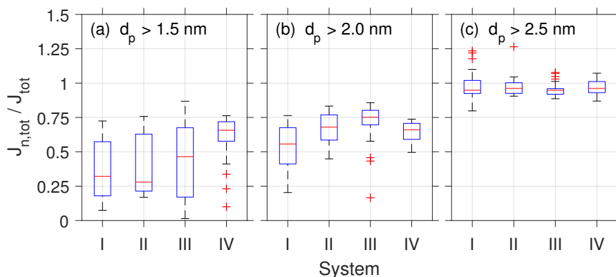
Figure 7. Comparison of the neutral fraction of particle formation rates for all four chemical systems at 5 °C and detection thresholds of (a) 1.5 nm, (b) 2.0 nm, and (c) 2.5 nm. The box and whisker plots show the median (red line), upper, and lower quartiles (rectangular box) and upper and lower ranges (error bars). Red crosses indicate outliers.
