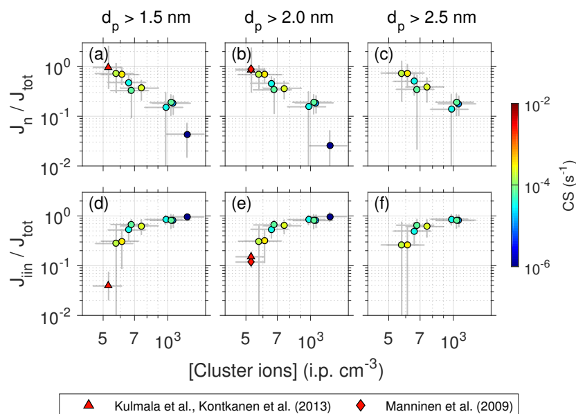
Figure 8. Comparison of CLOUD (system IV, circles) and Hyytiälä, Finland (triangles and diamonds), measurements of the neutral and ion-induced fractions of particle nucleation rates vs. cluster ion concentrations at 5 and 25 °C and detection thresholds of (a, d) 1.5 nm, (b, e) 2.0 nm, and (c, f) 2.5 nm. The color scale indicates the condensation sink (CS) onto aerosol particles (wall loss and dilution loss not included). The condensation sink in Hyytiälä is on average 2.5 \times 10^{-3} \text{ cm}^{-3} (Nieminen et al., 2014).
