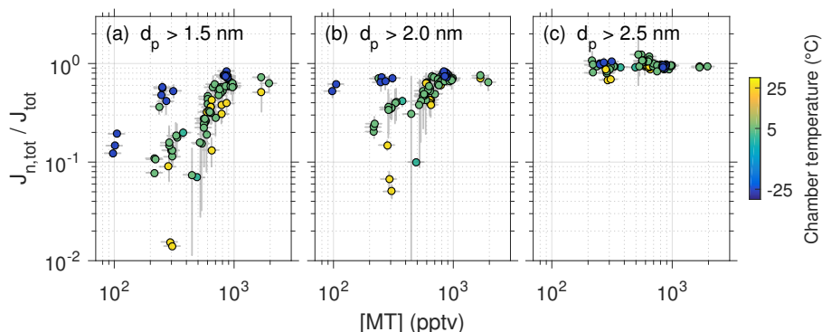
Figure 3. The neutral fraction of particle formation rates vs. monoterpene (MT) concentration for pure biogenic conditions (system I) at detection thresholds of (a) 1.5 nm, (b) 2.0 nm, and (c) 2.5 nm. The color scale indicates chamber temperature (−25, 5, 25 °C).
