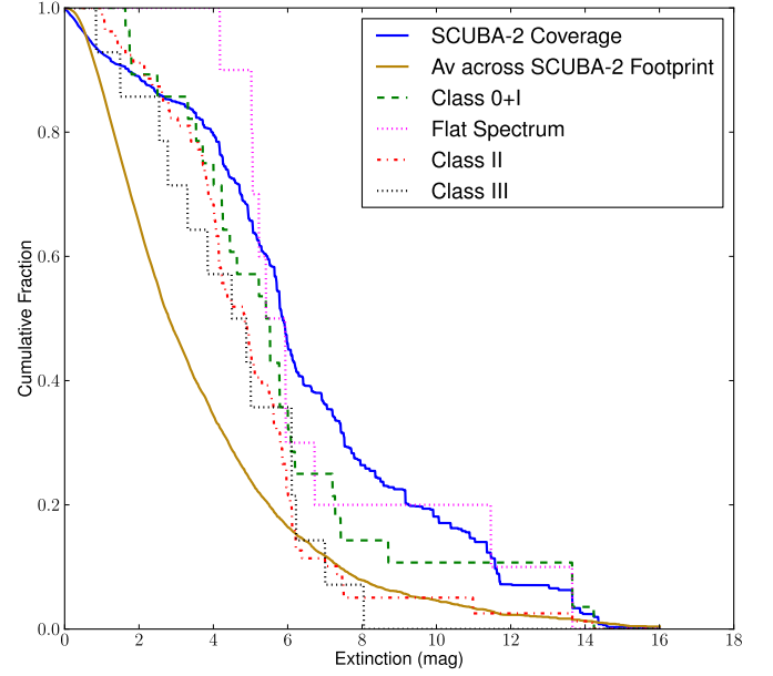
Figure 4. Cumulative mass as a function of extinction. The orange line plots the extinction-derived mass from the Cambréxy extinction map restricted to the SCUBA-2 areal coverage. The blue line plots the distribution of the submillimeter-derived mass from the 850\ \mu\text{m} SCUBA-2 map, as a function of the coincident Cambréxy extinction. The colored dash lines show the cumulative distributions of the YSOs, by Class, as a function of the coincident Cambréxy extinction.
