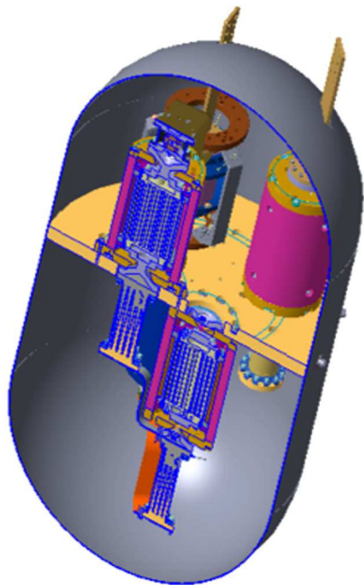
Fig. 21 The CADR under development at NASA GSFC. This will provide 6 \mu W of cooling at 50 mK. It also has a precooler stage that can be operated from 0.3 to 1.5 K. The picture also shows a notional enclosing magnetic shield for a <1 \mu T fringing field.
