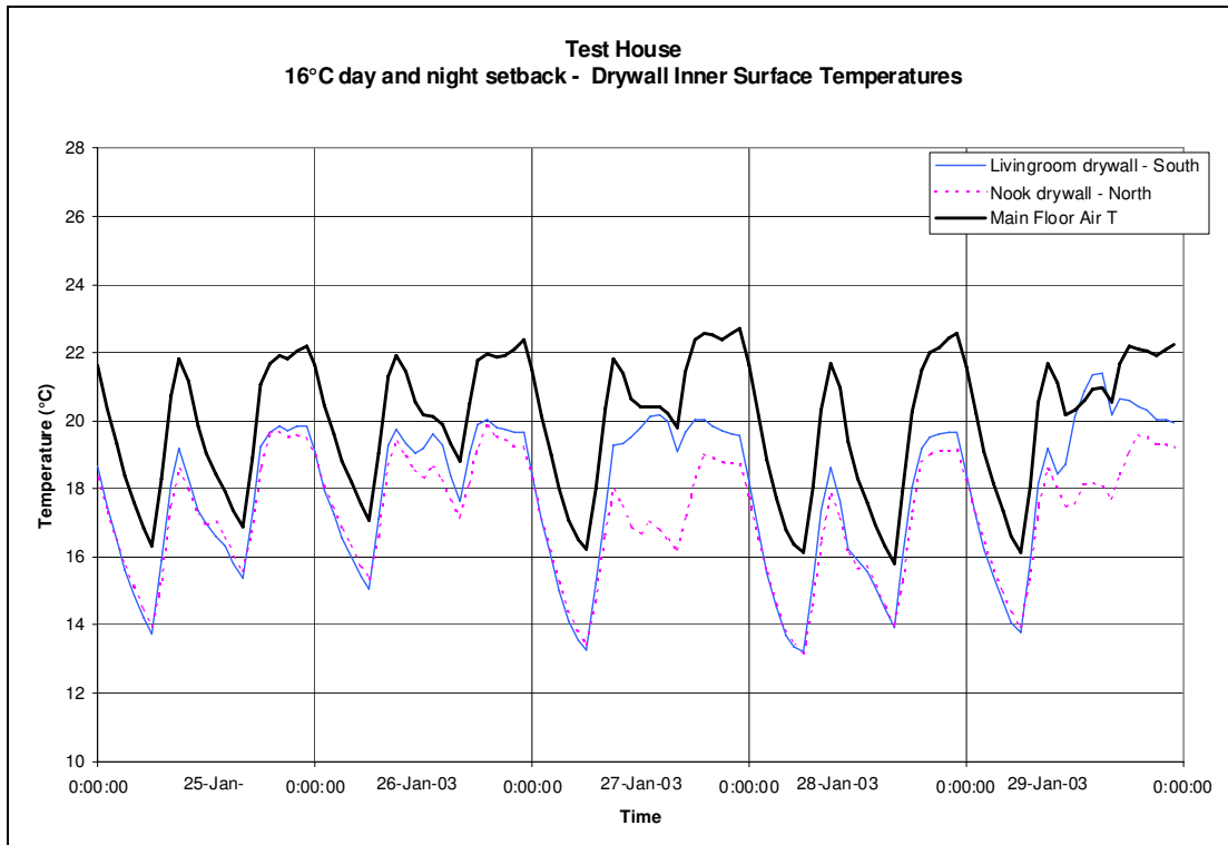
Figure 31 - Test House Air and Drywall Surface Temperature - 16°C Night and Day setback
