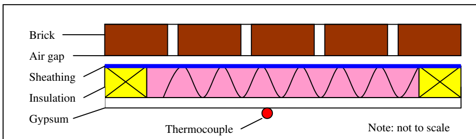
Figure 4 - Wall cross-section showing thermocouple location
