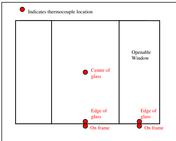
Figure 5 - Thermocouple Location on Window Inner Surface
