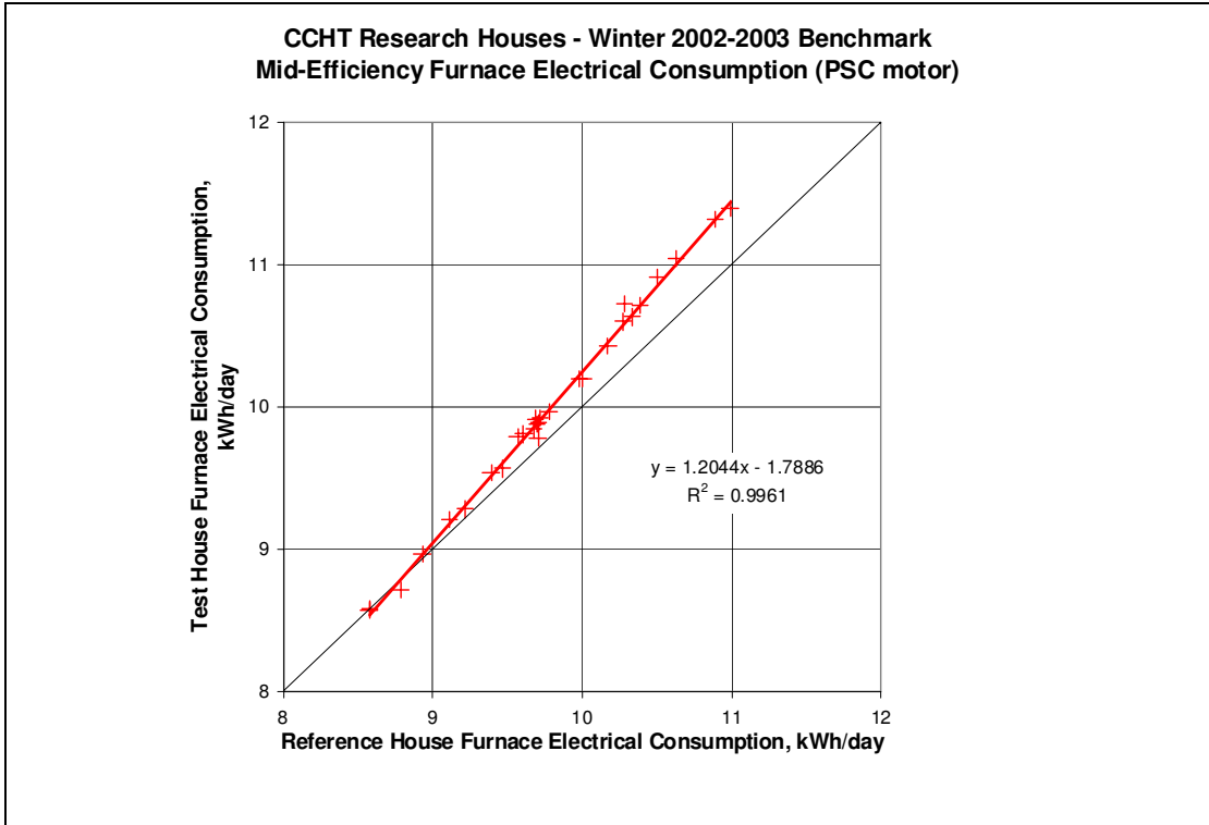
Figure 11 - Winter 2002-2003 Benchmark - Furnace Electrical Consumption
