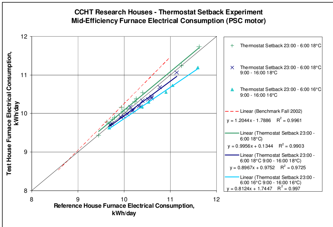
Figure 18 - Thermostat Setback Experiment - Furnace Electrical Consumption
