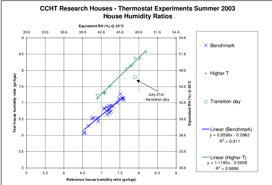
Figure 38 - House Humidity Ratios for Higher Temperature Setting
