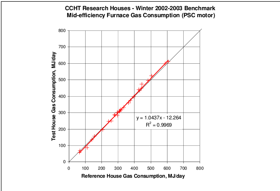
Figure 12 - Winter 2002-2003 Benchmark - Furnace Gas Consumption
