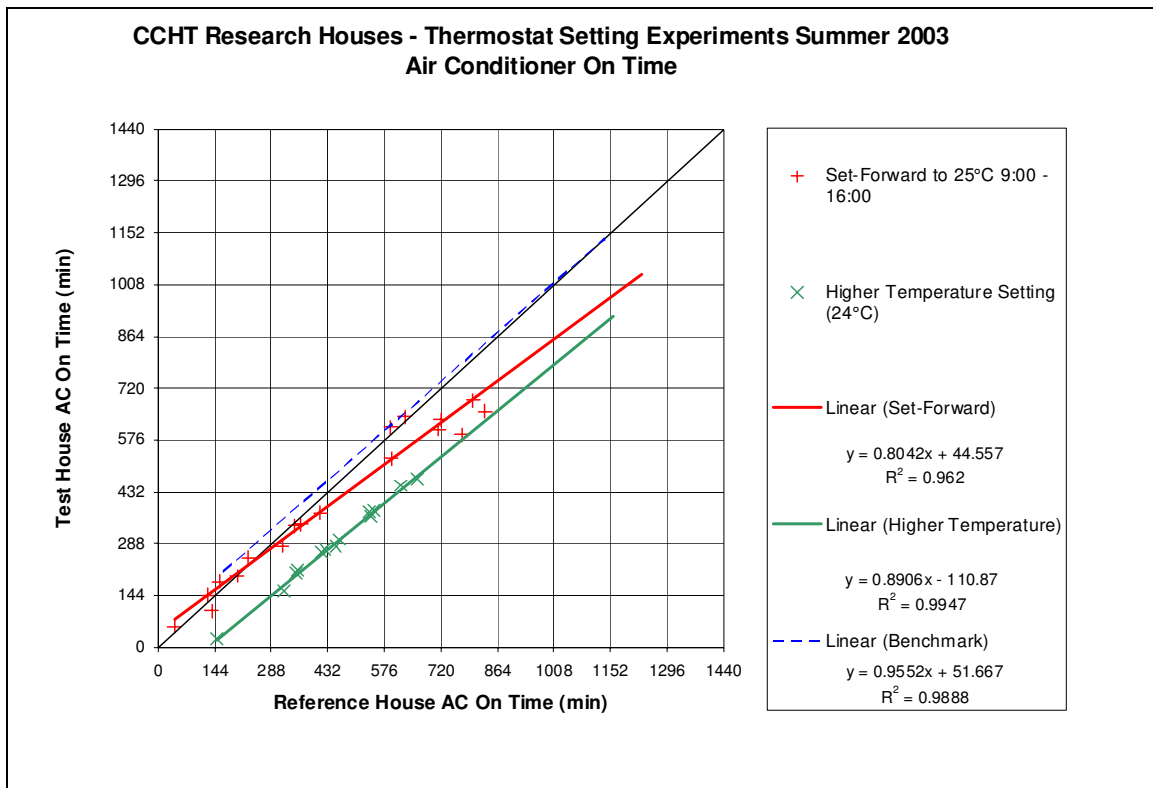
Figure 32 - Summer Thermostat Experiments - Air Conditioner On-Time
