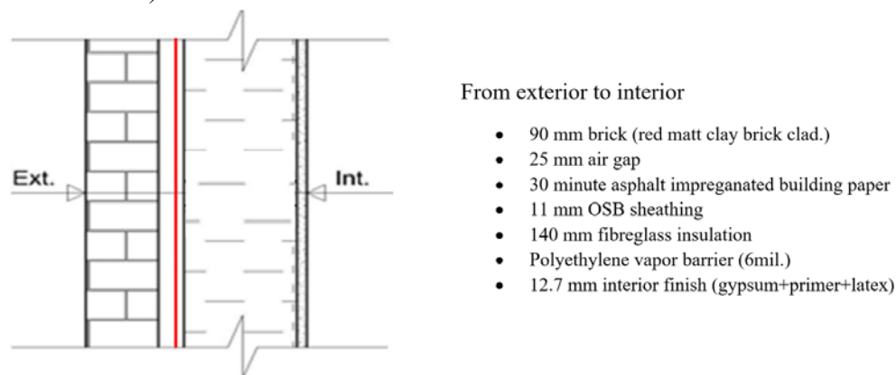
Figure 1. Cross-section of brick veneer cladding wood-stud wall assembly.
