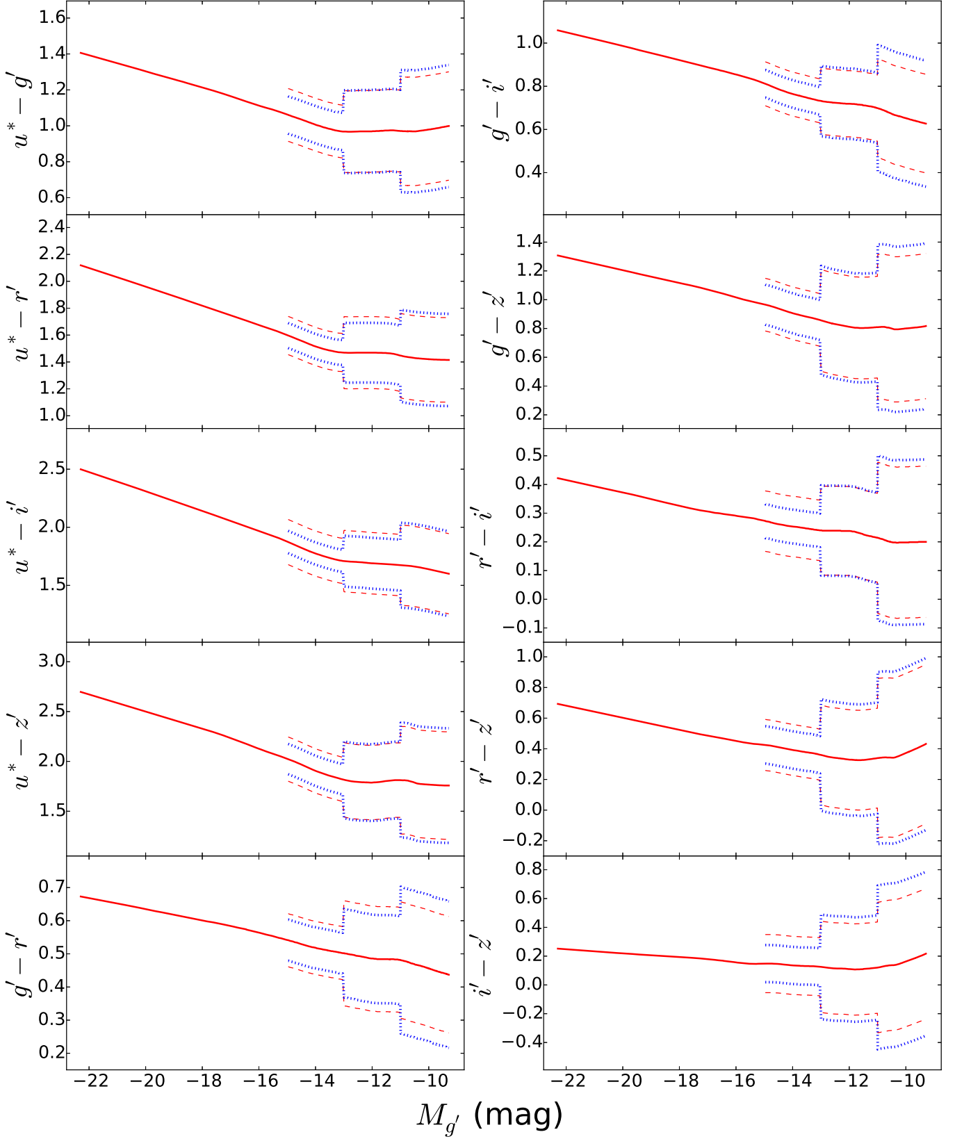
Figure 3. Comparison of the observed scatter [dashed lines] about the RS [solid lines] to photometric errors [dotted lines] established from artificial galaxy tests. The comparison is limited to M_{g'} \gtrsim -15 since our tests did not probe brighter magnitudes. The scatter and errors, averaged within three bins of luminosity, match quite well, especially at the faintest luminosities, suggesting minimal intrinsic scatter in the colors and stellar populations of these galaxies.
