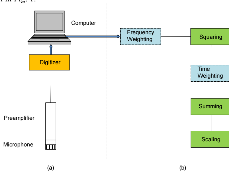
Figure 1 – A measurement system for ultrasound pressure level measurements. (a) Signal waveform recording unit with sound receiving device. (b) Post data processing unit.
