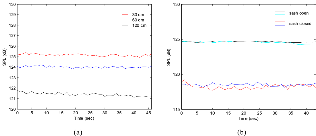
Figure 5 – Sound pressure level measurements for two setups. (a) Fig. 4a setup with microphone at the distances of 30 cm, 60 cm and 120 cm. (b) Fig. 4b setup with the fume hood sash open and closed.
