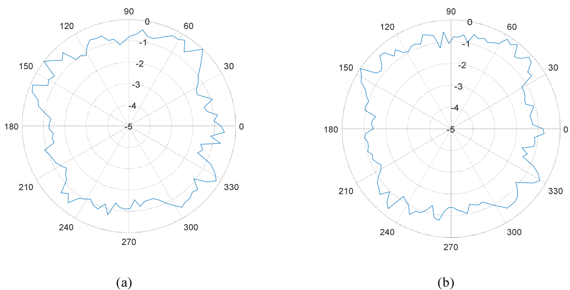
Figure 3 – Beam patterns of an ultrasound source. (a) On a horizontal plane (base plane of cleaner). (b) On a 60° cone with the apex at the acoustic center of the source.
