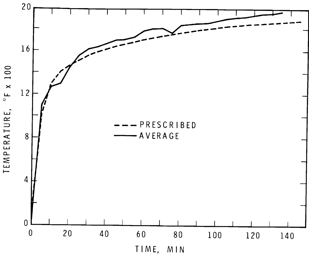
FIGURE 8 FURNACE TEMPERATURE, TEST NO. 1
