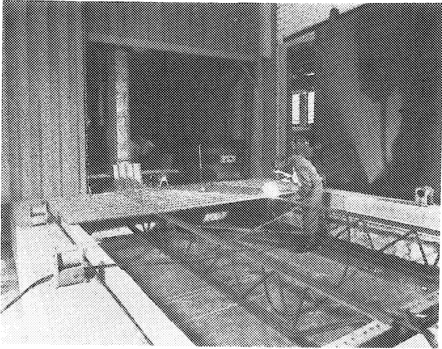
FIGURE 19 DECK INSTALLATION
