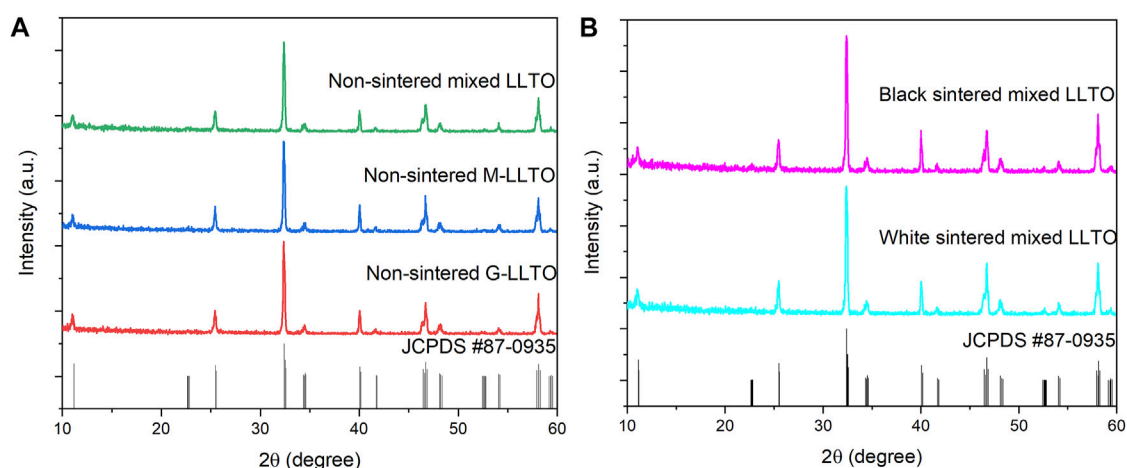
FIGURE 3 2D stacked XRD spectra of: (A) non-sintered LLTO pellets; and (B) sintered mixed LLTO pellets.
