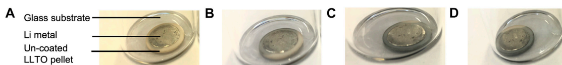
FIGURE 2 Photographs of LLTO contacts with Li-metal after: (A) 5 min; (B) 30 min; (C) 60 min; and (D) 90 min.
