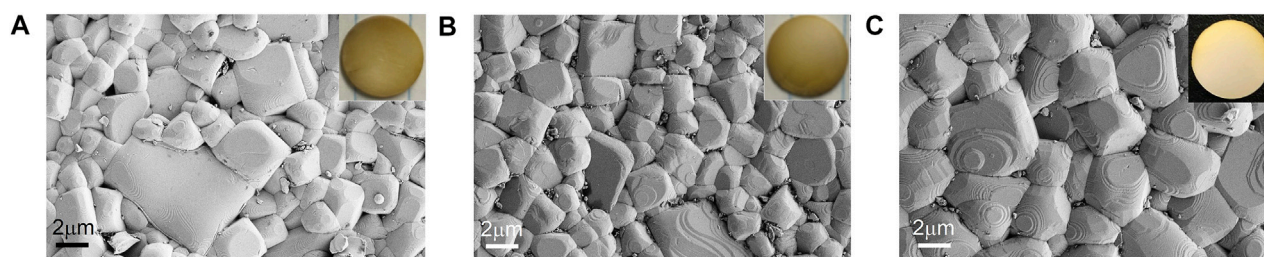
FIGURE 1 SEM pictures of sintered pellets (without polishing) at 1,170°C for 12 h in air: (A) G-LLTO; (B) M-LLTO; and (C) mixed LLTO.
