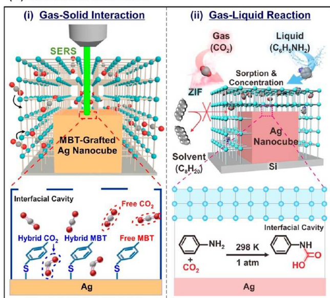
Figure 48. Emerging strategies to monitor liquid-based (A) and gas-based (B) reactions using SERS. (A) Particle-assembled microdroplets, such as plasmonic liquid marble and plasmonic colloidosome, have been designed to track (i) immiscible liquid–liquid reactions; adapted from ref 955, Copyright 201, American Chemical Society; and (ii) electrochemical reactions; adapted with permission from ref 955, copyright 2016 Wiley-VCH. (B) Integrating MOFs with SERS to read-out molecular events during (i) gas–solid interaction; adapted from ref 958, copyright 2017 American Chemical Society; (ii) gas–liquid reaction; adapted with permission from ref 959, copyright 2018, Wiley-VCH.
