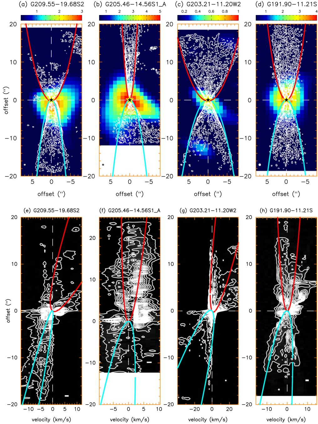
Figure 2. Panels (a) to (d): CO channel maps (contours) and C^{18}O total intensity maps (color image) for the four ALMASOP sources G209 (HOPS 10), G205 (HOPS 358), G203, and G191. The contour levels start at 3\sigma with a step of 3\sigma , and the \sigma are \sim 0.013 , 0.016 , 0.013 and 0.016 \text{ Jy beam}^{-1} \text{ km s}^{-1} in panels (a) to (d), respectively. The yellow-black stars denote the central source position. Panels (e) to (h): CO PV diagrams cut along the outflow axis for the four sources. The contour levels start at 10\sigma with a step of 10\sigma , and \sigma are \sim 0.002 , 0.0012 , 0.001 , and 0.002 \text{ Jy beam}^{-1} in panels (e) to (h), respectively. The blue and red curves are the fits to the structures and PV structures of the outflows from the wind-driven shell model (see Section 3.2).
