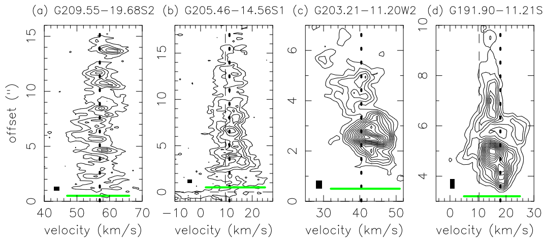
Figure B1. PV diagrams of the jets along the jet axis in SiO. The width of the green line segment denotes the observed radial sideways-ejection velocity ( \Delta V_{\text{obs}} ) for each source, and the dotted line denotes the observed radial jet velocity ( V_{\text{obs}} ). The contour levels start at 3\sigma with a step of 3\sigma , and \sigma are \sim 0.002 , 0.002 , 0.002 , and 0.0019 Jy beam ^{-1} in panels (a) to (d), respectively.
