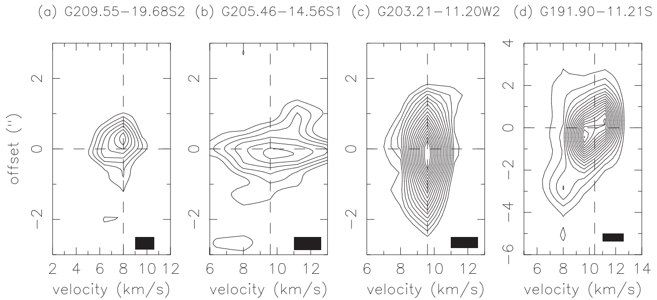
Figure A1. PV diagrams cut perpendicular to the jet axis going through the sources' center for four sources (G209, G205, G203, and G191) in C^{18}O , centered at the source position. The contour levels start at 3\sigma with a step of 3\sigma , and \sigma are \sim 0.003 , 0.003 , 0.003 , and 0.003 Jy\ beam^{-1} in panels (a) to (d), respectively. The vertical dashed line indicates the systemic velocity for each source.
