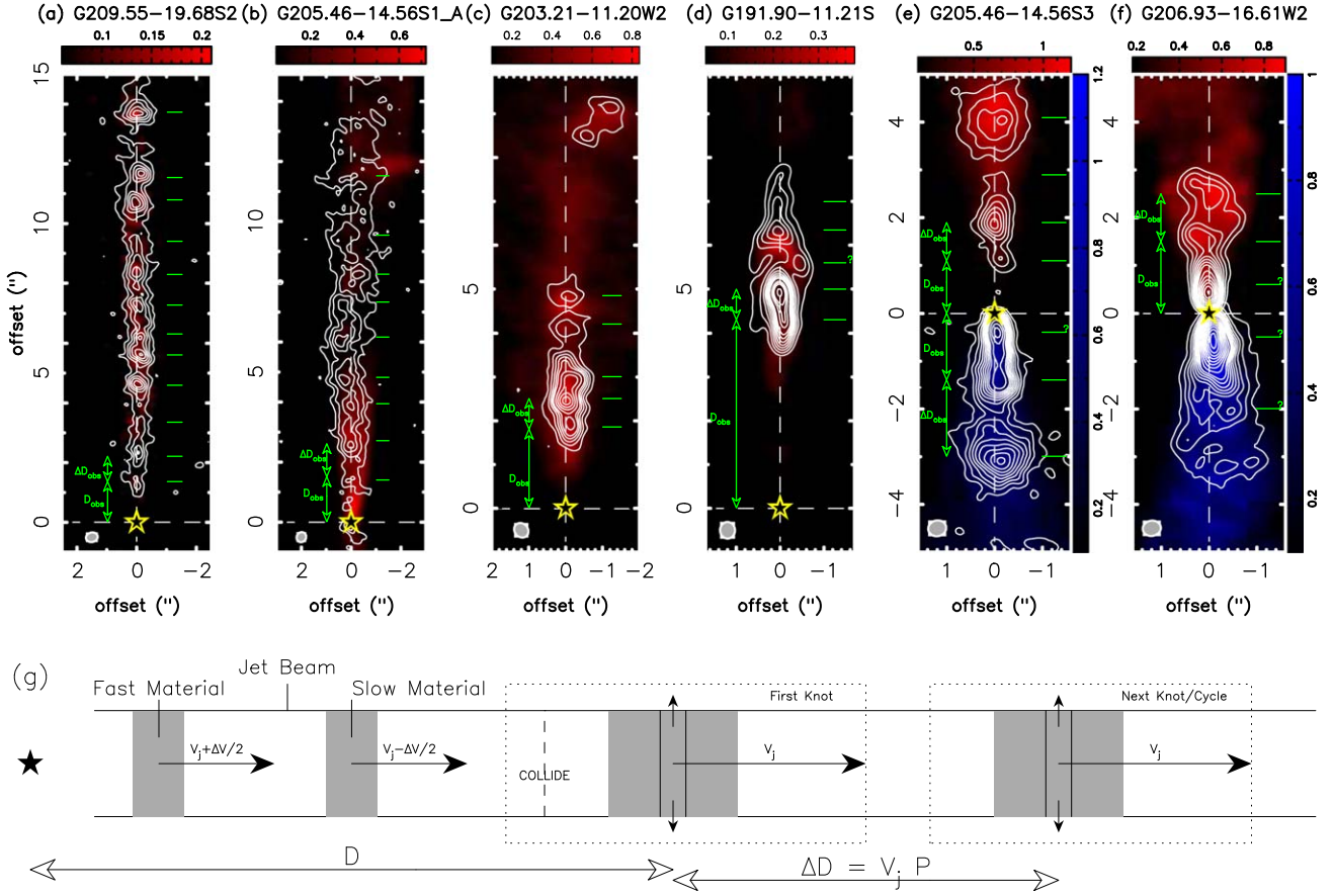
Figure 1. Panels (a) to (f): CO (red color for redshifted and blue color for blueshifted) intensity maps and SiO (white contour) intensity maps for the six ALMASOP sources, G209 (HOPS 10), G205 (HOPS 358), G203, G191, G205S3 (HOPS 315), and G206 (HOPS 399). These maps have been rotated clockwise by 29^\circ , 158^\circ , 146.7^\circ , -5^\circ , -135^\circ , and -20^\circ , respectively, to align the jets with the vertical axis. For SiO, the contour levels start at 3\sigma with a step of 3\sigma , and \sigma are \sim 0.02 , 0.04 , 0.01 , 0.02 , 0.03 , and 0.06 \text{ Jy beam}^{-1} \text{ km s}^{-1} in panels (a) to (f), respectively. The green line segments indicate the SiO peak positions of the knots. The yellow-black stars denote the central source position. The green arrows mark the lengths of D_{\text{obs}} and \Delta D_{\text{obs}} . Panel (g): Schematic diagram showing how fast and slow jet material interact to form the internal shocks seen as knots (Raga et al. 1990; Stone & Norman 1993; Suttner et al. 1997; Lee & Sahai 2004; Jhan & Lee 2016).
