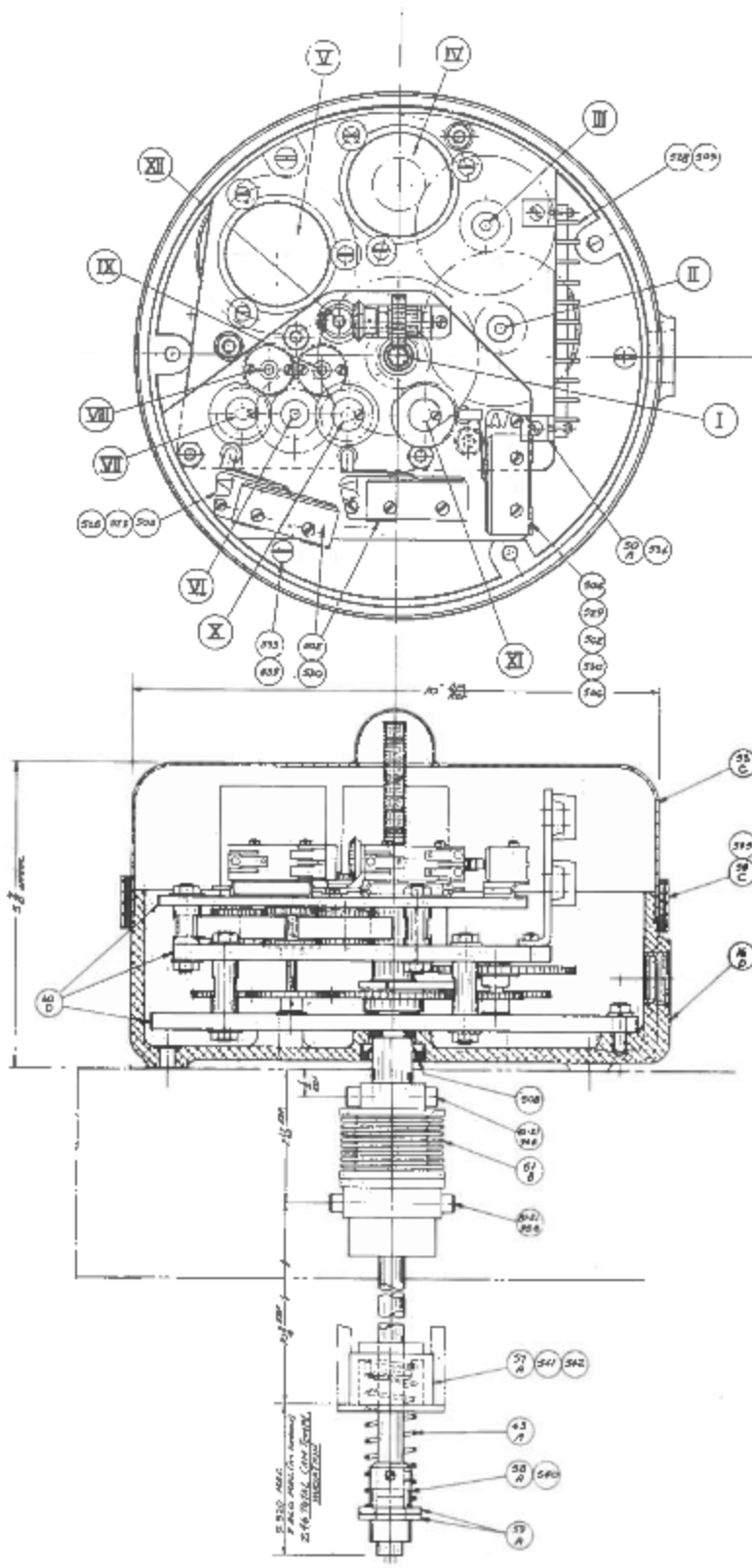
Fig. 2 Polar-axis data gear box
