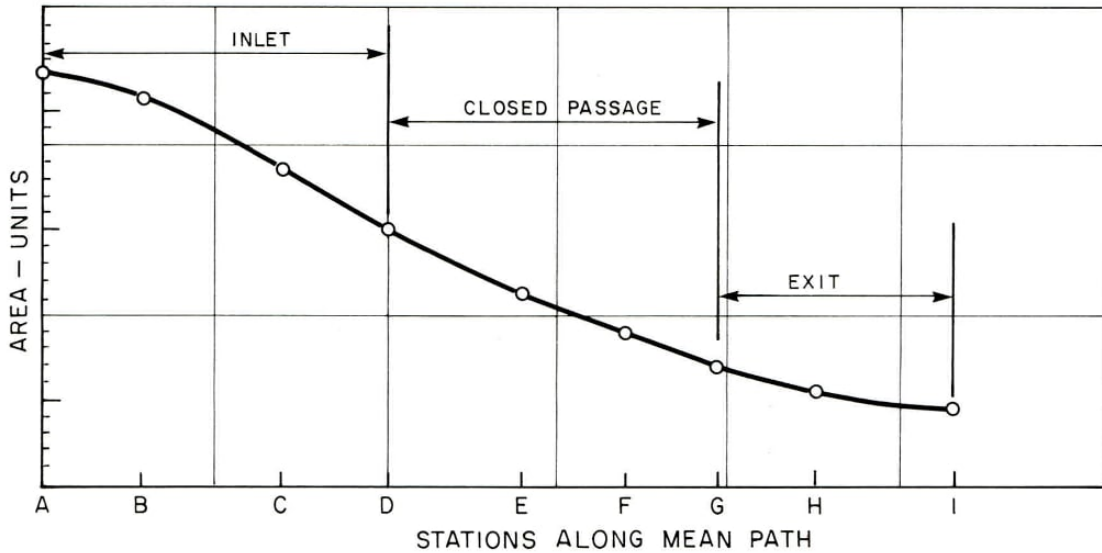
FIG. C-2: BLADE "E" - TWO SLOTS
