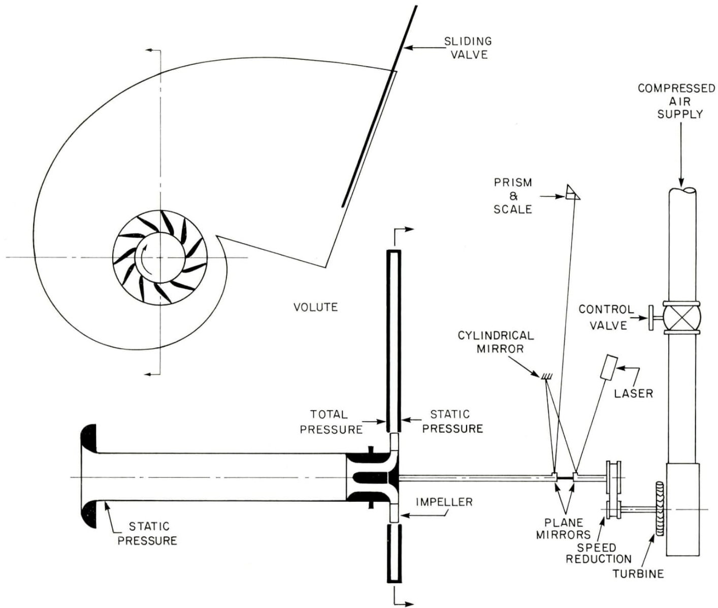
FIG. 10: DIAGRAM OF HIGH SPEED CENTRIFUGAL COMPRESSOR RIG
