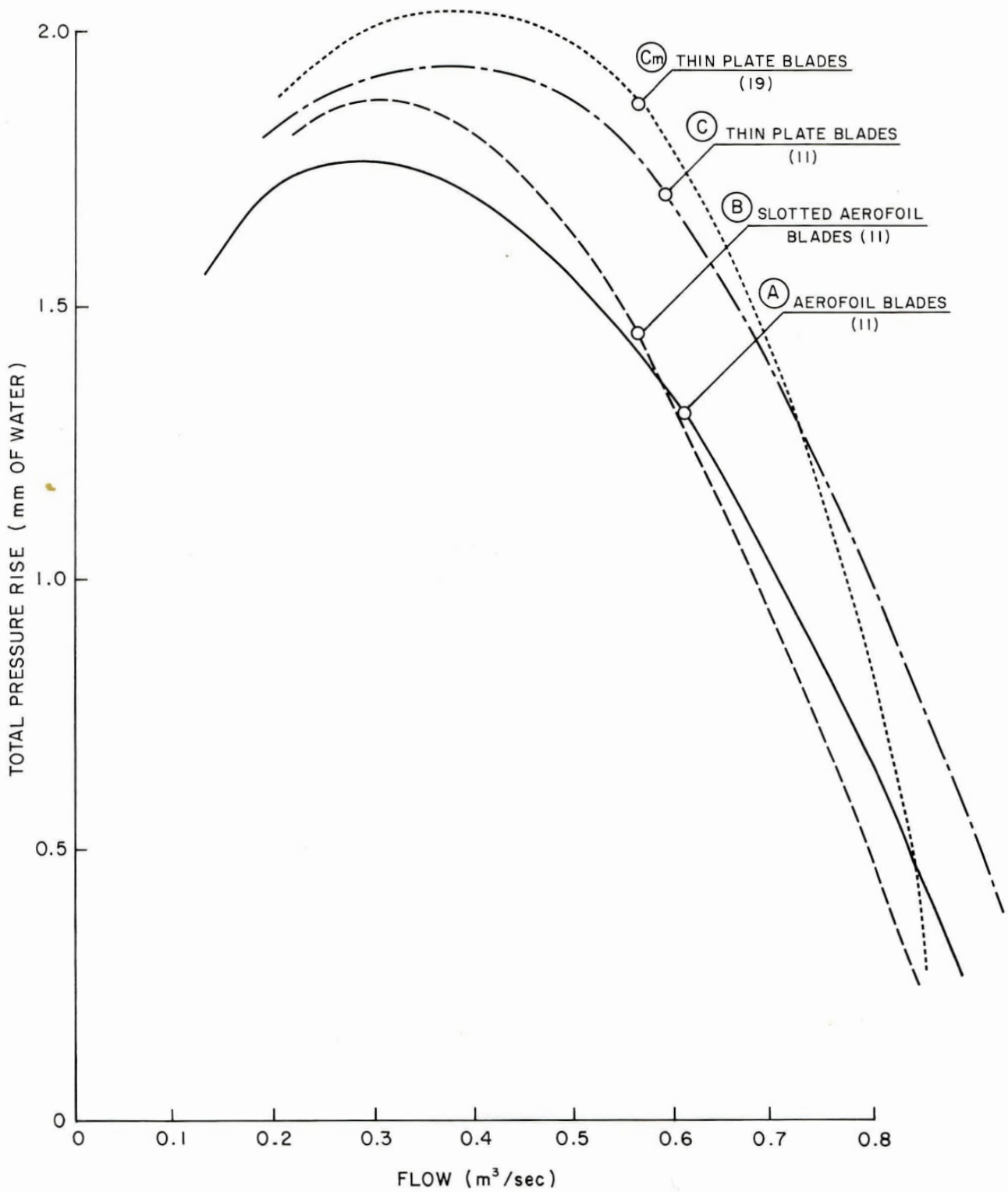
FIG. 4: PRESSURE RISE ~ FLOW CHARACTERISTICS (70 RPM) BLADE SET VB2 [STRAIGHT BLADES] VARIANTS A, B, C, Cm
