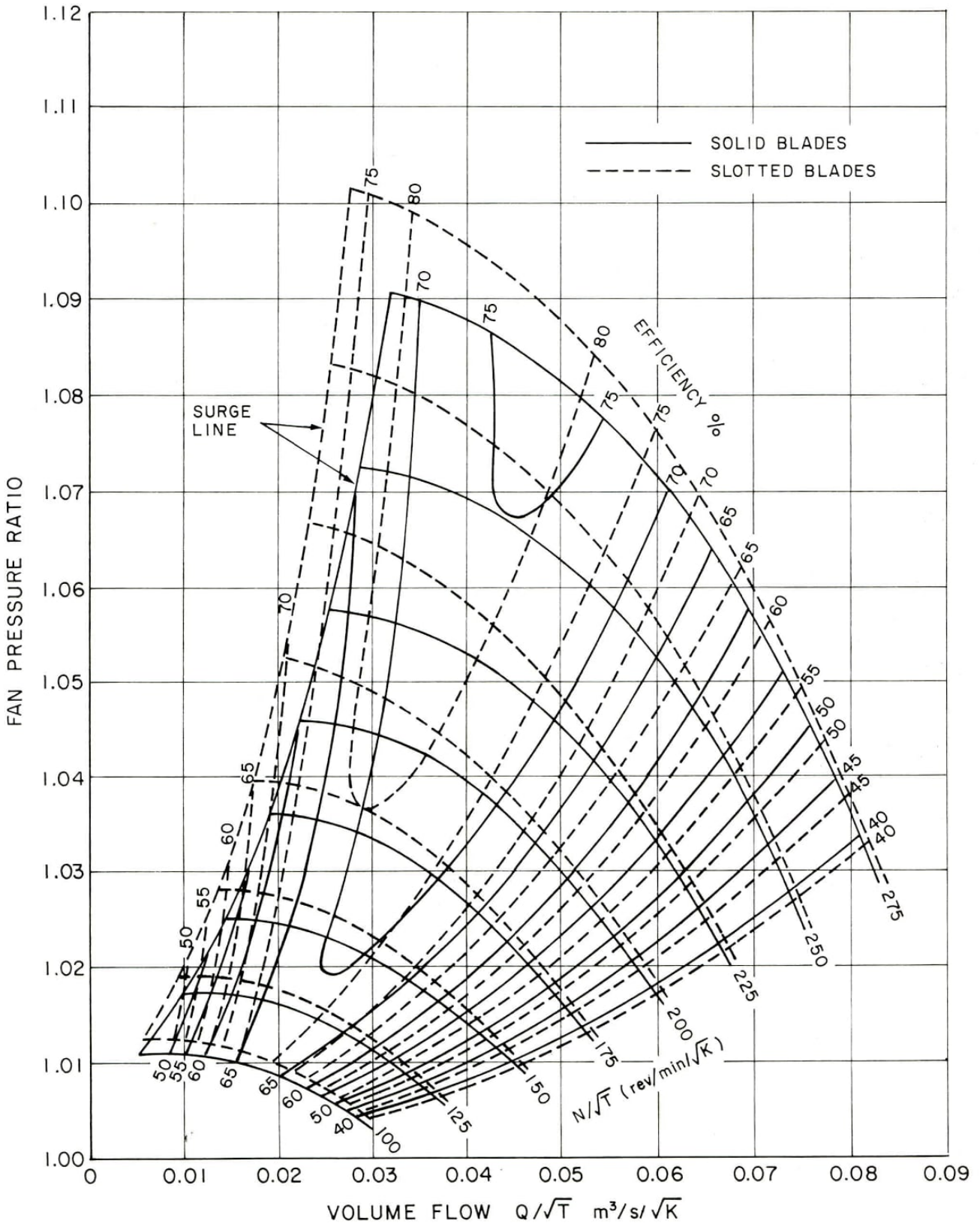
FIG. 12: FAN PERFORMANCE (HIGH SPEED RIG)
