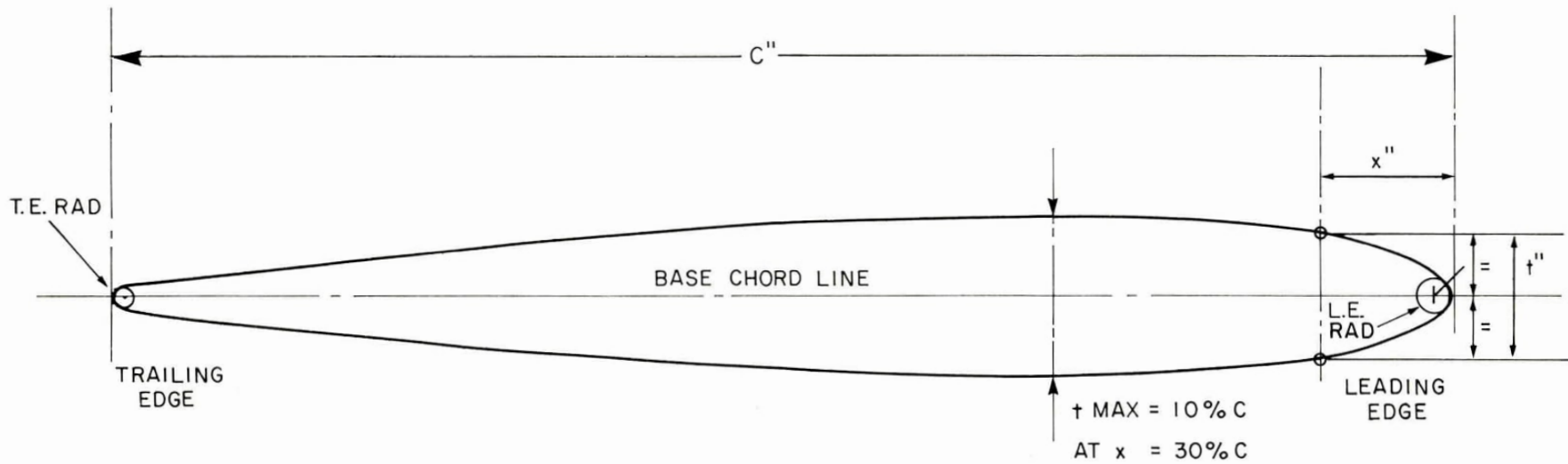
ORDINATES FOR C-4 AEROFOIL WITH t/c_{MAX} = 10\%
