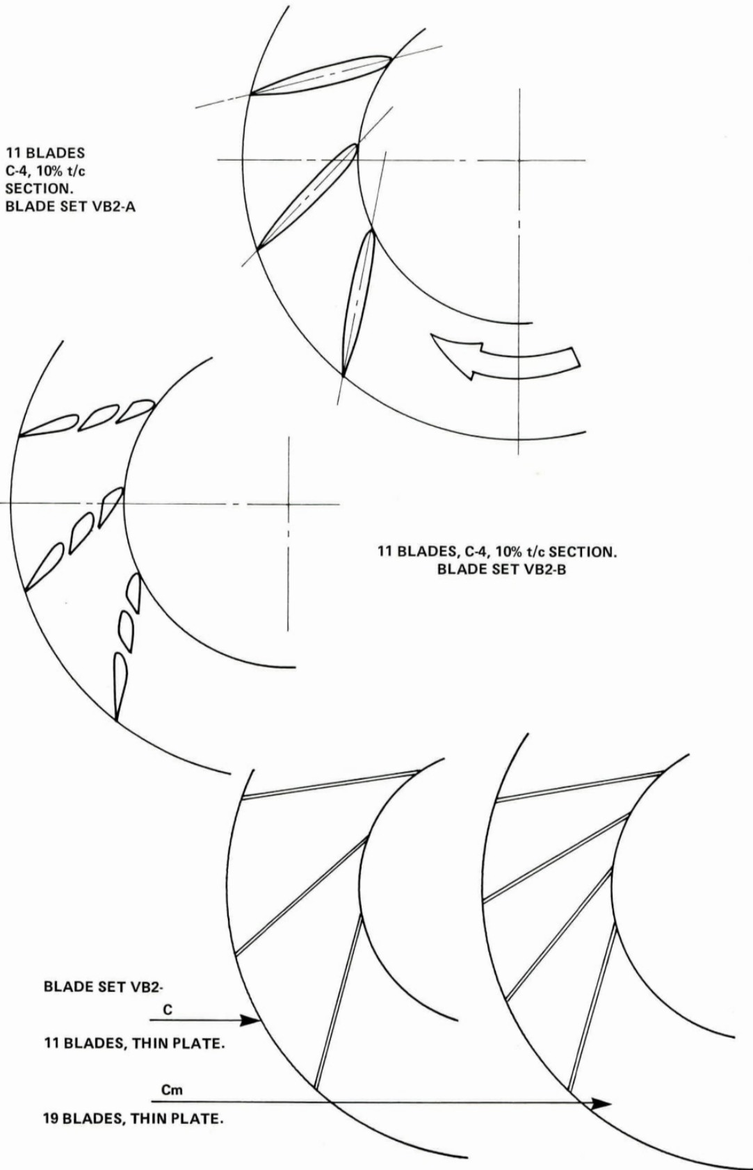
FIG. B-4: BLADE SETS VB2-A, B, C, AND Cm
