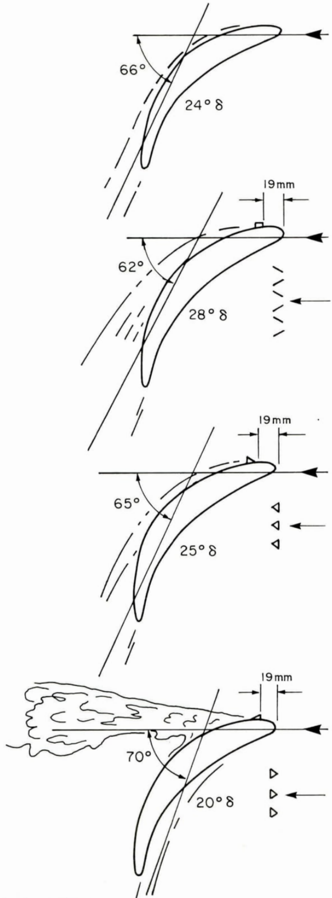
FIG. A-4: STATIC TESTS (VORTEX GENERATORS)
