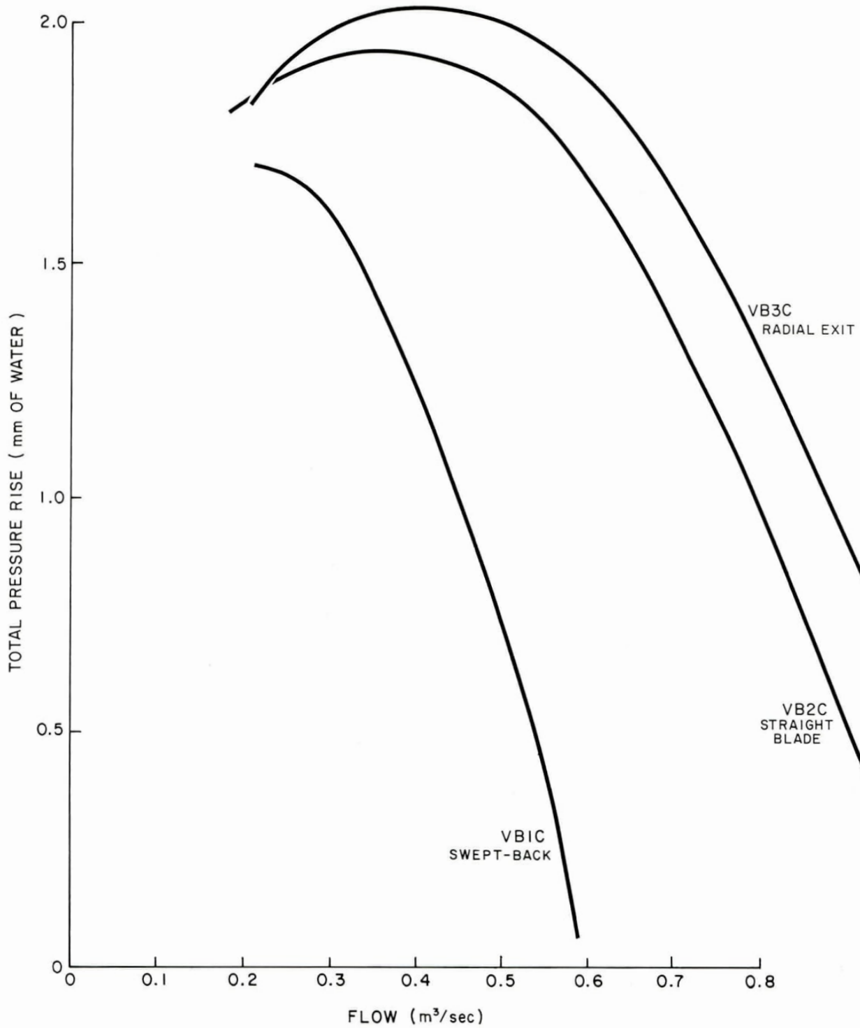
FIG. 8: PRESSURE RISE ~ FLOW CHARACTERISTICS (70 RPM) VARIANT © – THIN PLATE BLADES, SETS VB1, 2 & 3
