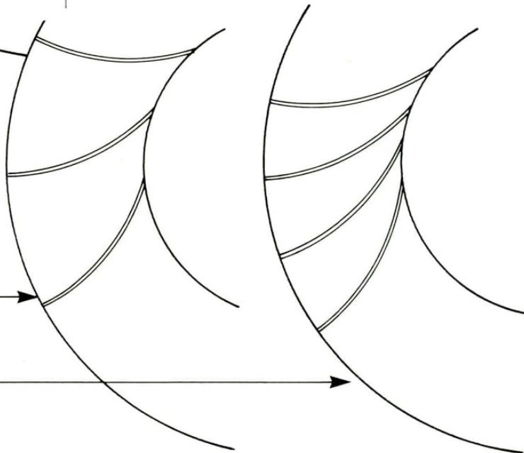
FIG. B-5: BLADE SETS VB3-A, B, C, AND C m
