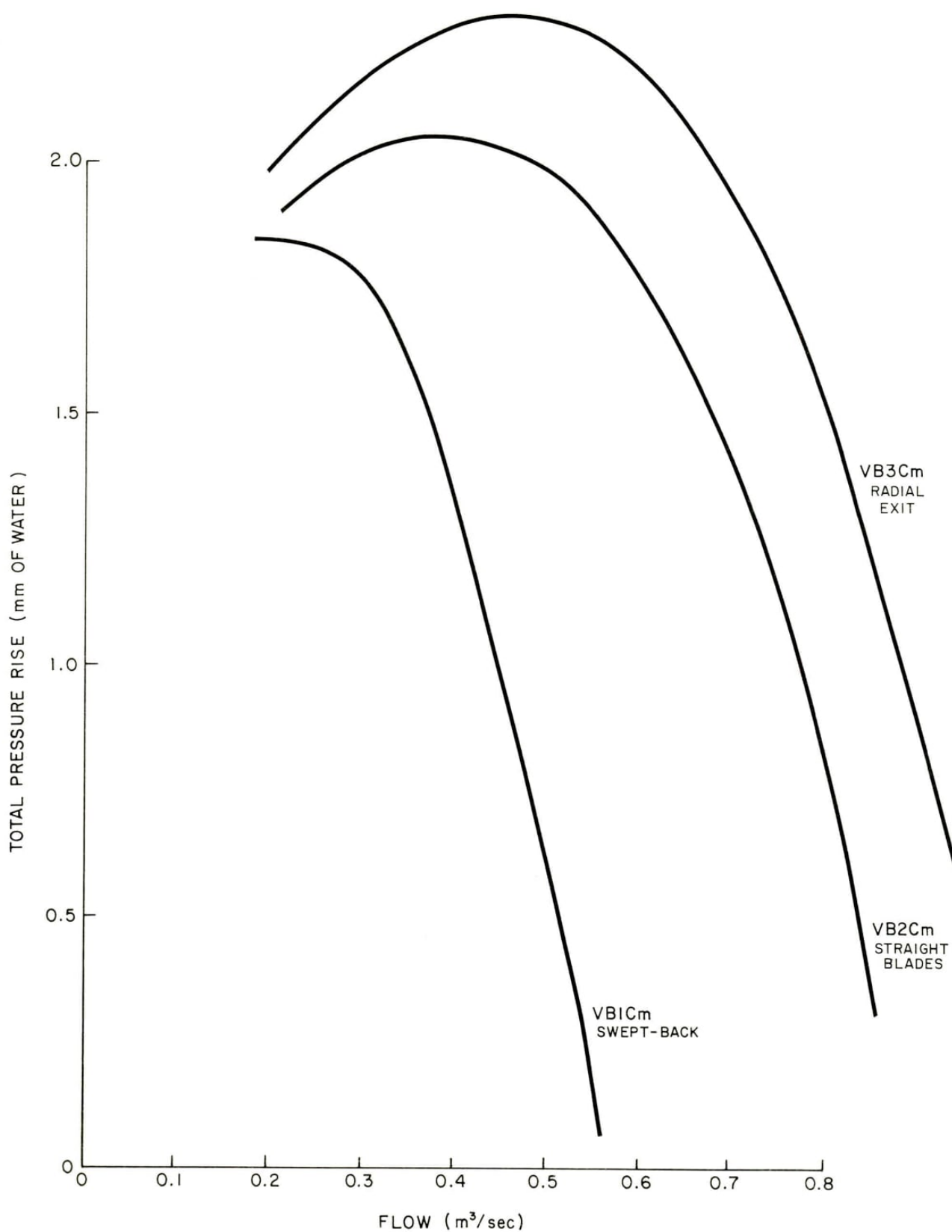
FIG. 9: PRESSURE RISE ~ FLOW CHARACTERISTICS (70 RPM) VARIANT \text{C}_m - THIN PLATE BLADES (CLOSELY SPACED), SETS VB1, 2 & 3
