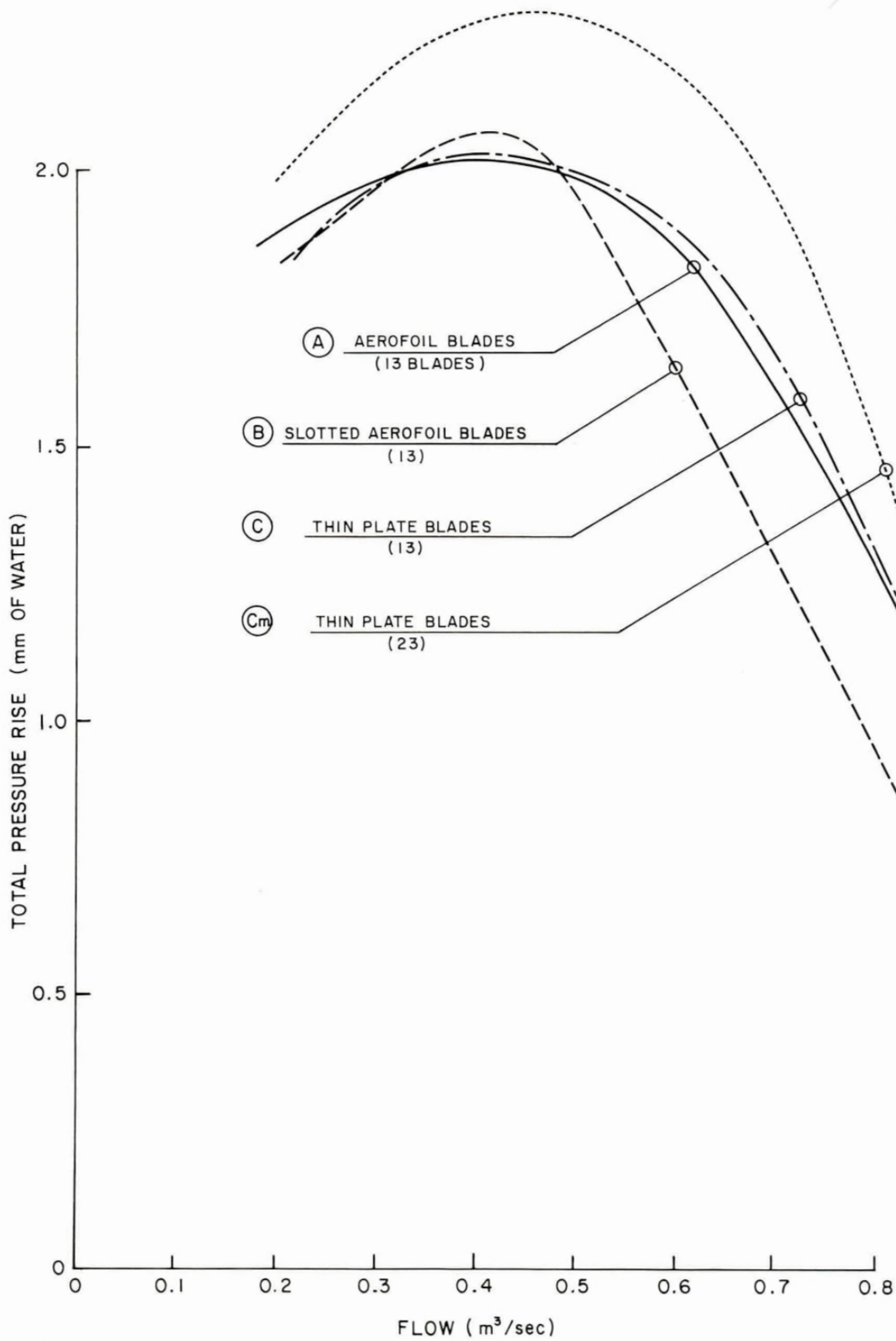
FIG. 5: PRESSURE RISE ~ FLOW CHARACTERISTICS (70 RPM) BLADE SET VB3 [RADIAL EXIT BLADES] VARIANTS A, B, C, Cm
