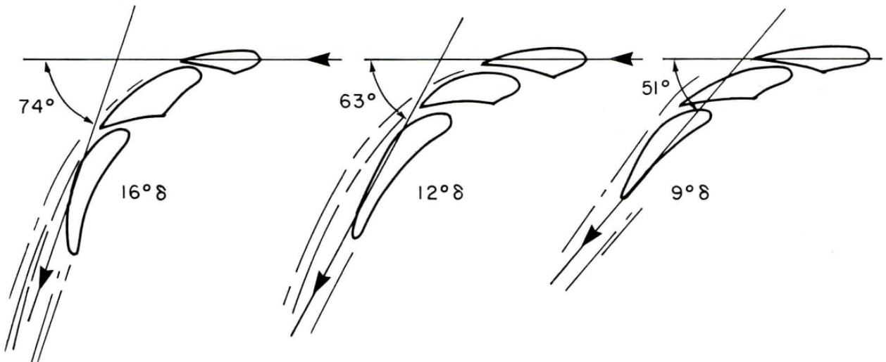
FIG. A-2: STATIC TESTS (VARIOUS SLOTTED BLADES)
