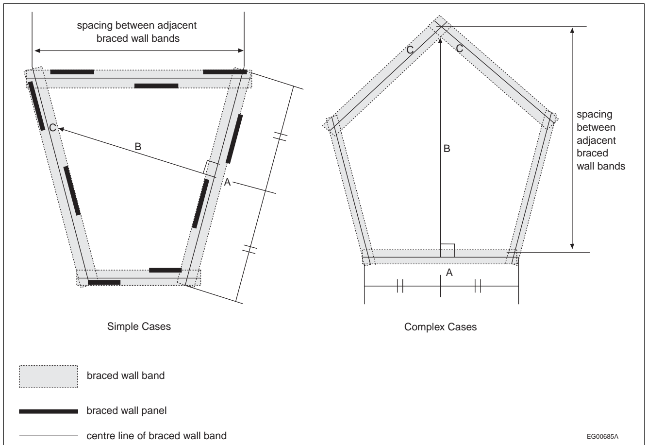
Figure Table A-9.23.13.5.-B Identification and spacing of adjacent non-parallel braced wall bands
