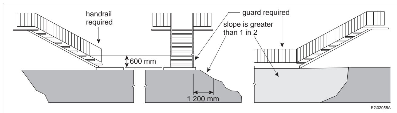
Figure A-9.8.8.1. Required locations of guards
