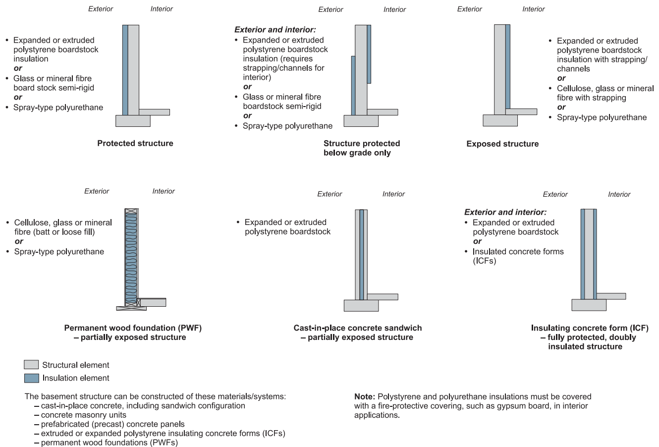
Figure 1. Typical arrangements of structural and insulation elements
