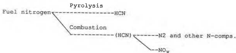
Figure 2 Hypothesis for \text{NO}_x and HCN Generation
