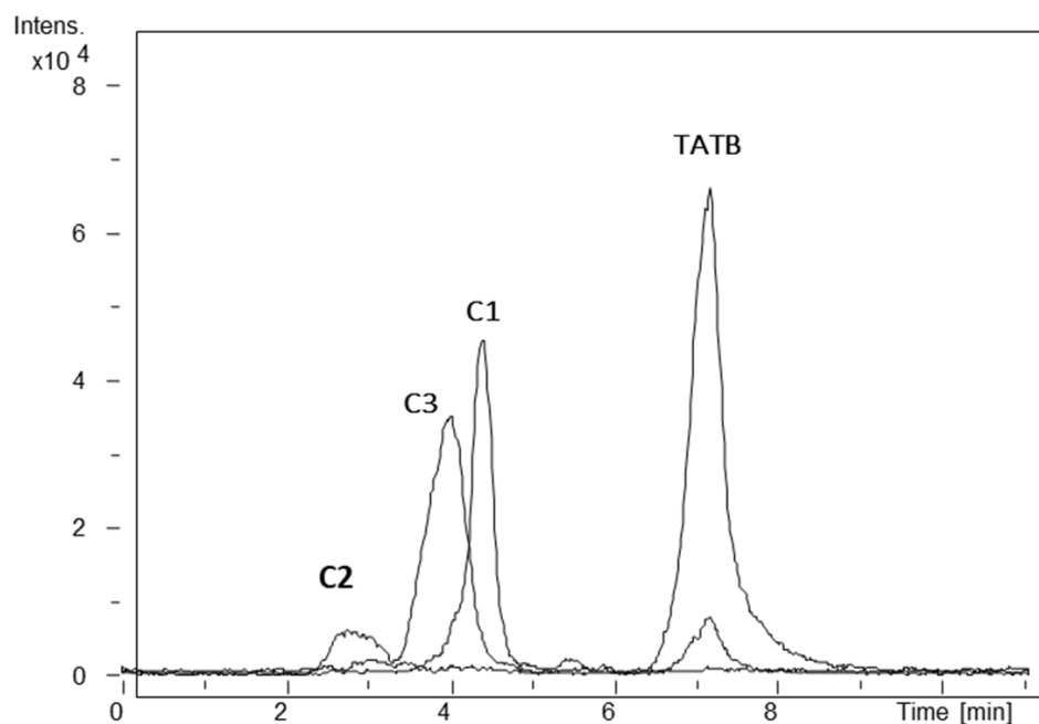
Figure 2. Extracted ion chromatograms (EICs) at m/z 239 (C1), m/z 257 (C2 and TATB), and m/z 258 (C3) of the acetonitrile extracts of TATB (54 mg) photolyzed in a SolSim photoreactor for 6 days.
