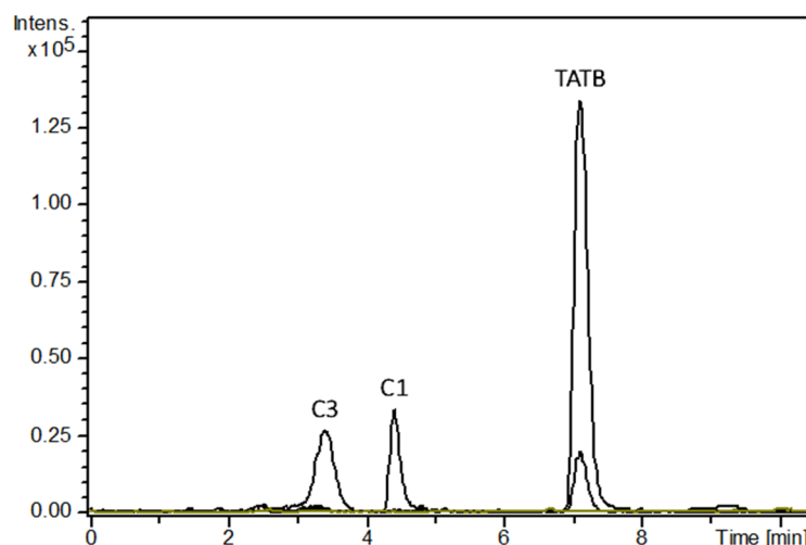
Figure 4. Extracted ion chromatograms (EICs) at m/z 239 (C1), m/z 257 (TATB) and m/z 258 Da (C3) of DMSO extract of TATB (2.5 mg) photolyzed in a SolSim photoreactor for 4 days and analyzed 6 months later, showing the absence of the aci -nitro isomer of TATB.
