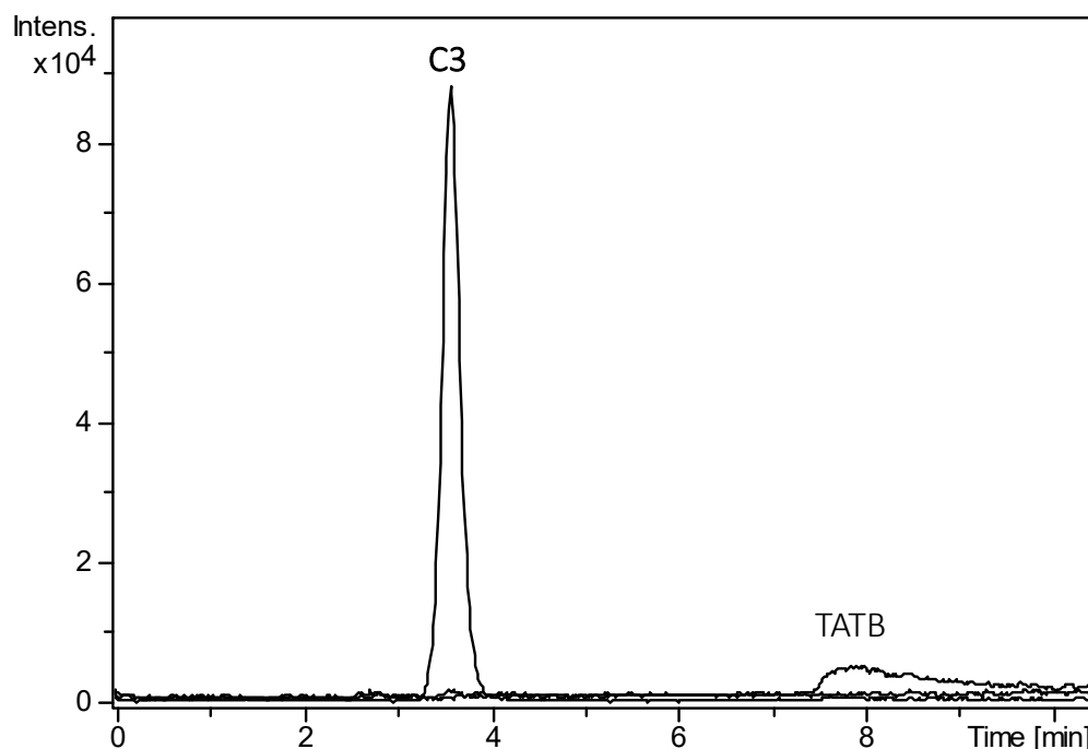
Figure 3. Extracted ion chromatograms (EICs) at m/z 257 (TATB) and m/z 258 (C3) of TATB in water incubated at 50 °C for 8 days.
