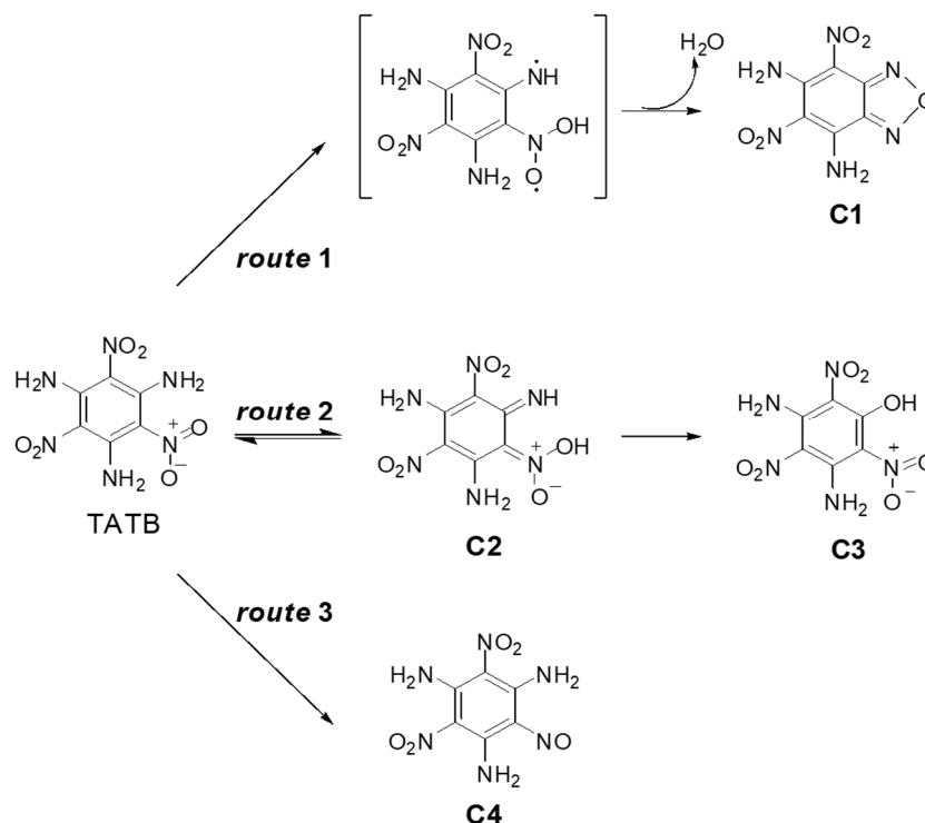
Scheme 1. Postulated major (1) initial route involved in the photodegradation of TATB under both simulated sunlight and UV at 254 nm. The structure of compound in bracket was originally proposed by Wu and Fried [15]. Two minor routes, (2) and (3), were observed only under simulated sunlight and UV at 254 nm, respectively.
