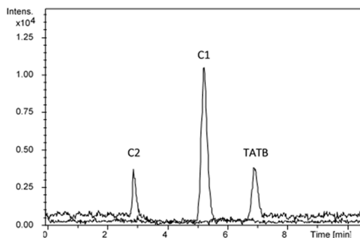
Figure 1. (top) UV and MS [M - H]^- spectra of TATB standard ( 0.273 \text{ mg L}^{-1} in 50% acetonitrile in water); (bottom) extracted ion chromatograms (EICs) at m/z 239 (C1) and m/z 257 (C2 and TATB) of DMSO extract of TATB (2.1 mg) photolyzed in a SolSim photoreactor (280–800 nm) for 4 days.
