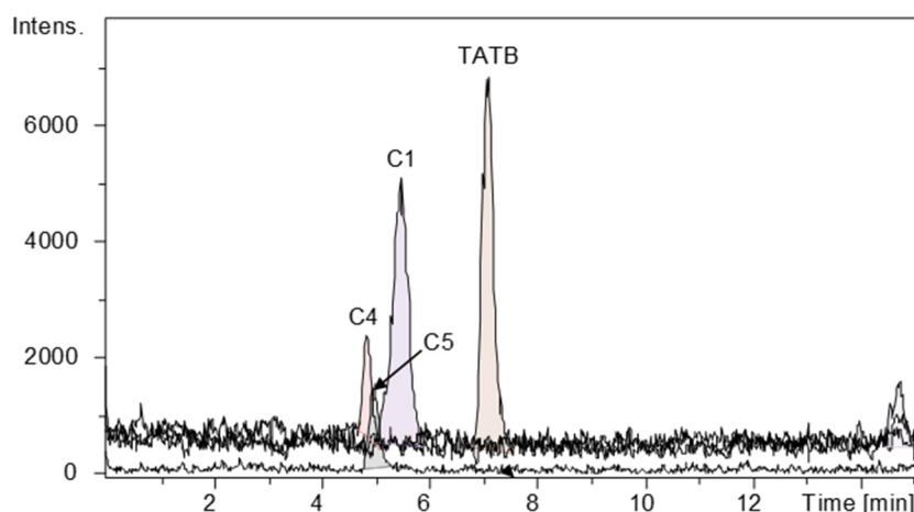
Figure 5. Extracted ions chromatograms (EICs) at m/z 241 (C4), m/z 212 (C5), m/z 239 (C1) and m/z 257 (TATB) of the sample ( 0.7 \text{ mg L}^{-1} ) prepared in MeCN-50 (1:1 ( v/v ) mixture of water and acetonitrile) and photolyzed at 254 nm for 10 min.
