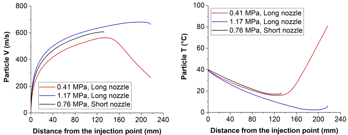
Fig. 8 Simulated inflight particle (20 \mu\text{m} ) velocity and temperature from injection point to impact along the centerline of the short and long nozzles for selected spray conditions
