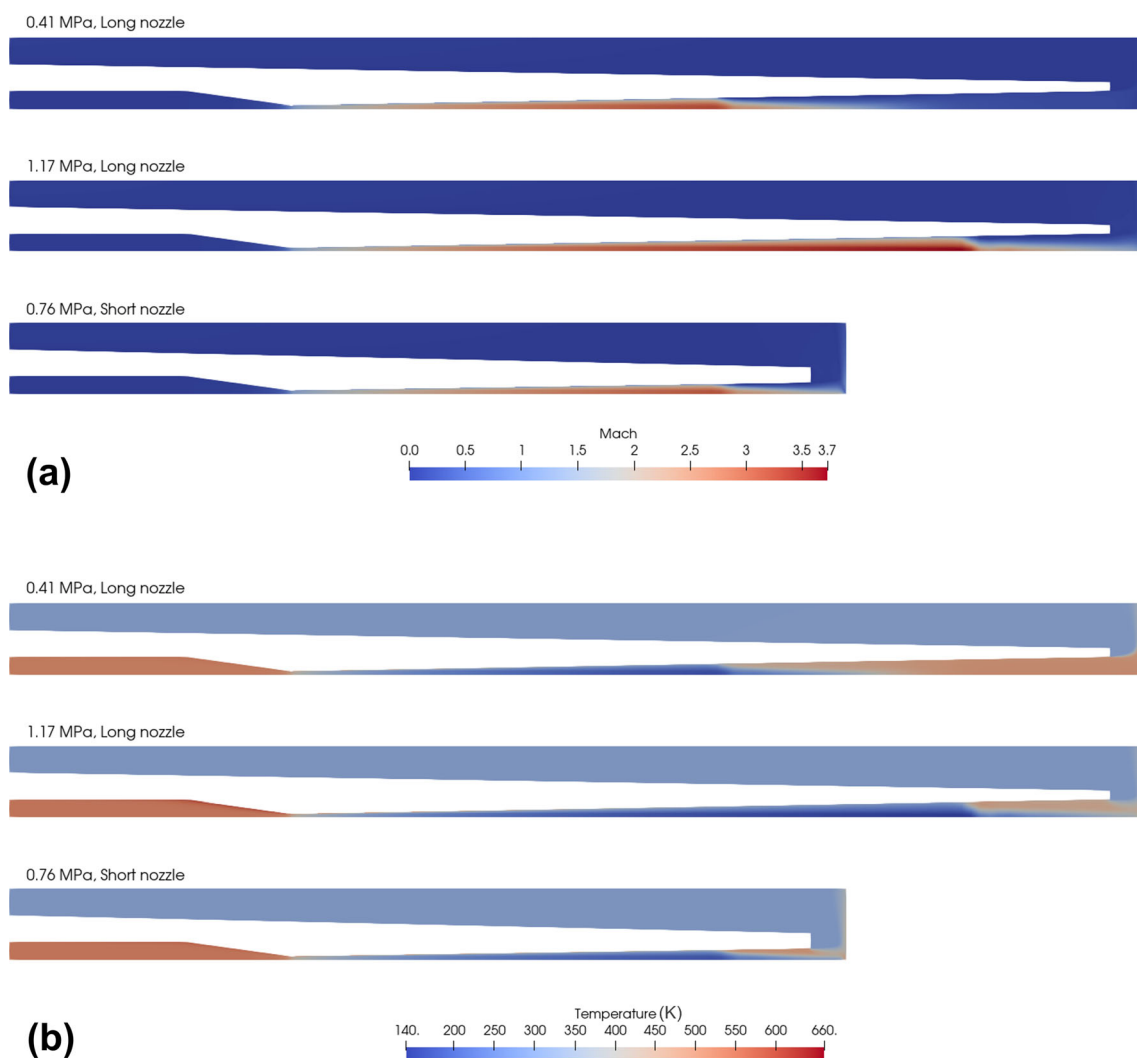
Fig. 9 (a) Mach number and (b) temperature along the domain for three selected conditions
