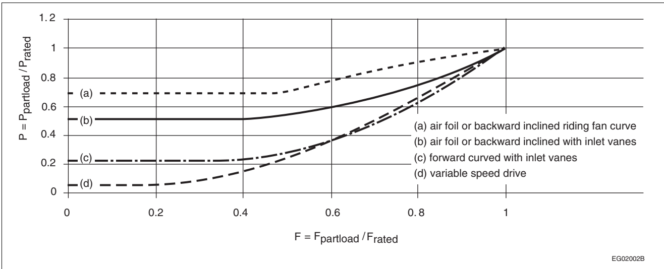
Figure A-8.4.17.(2) Fan part-load curves
