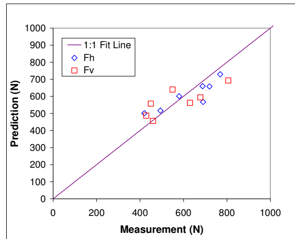
Figure 6: Comparison of model predictions with force measurements from C-CORE's centrifuge tests with freshwater ice
