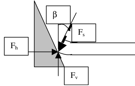
Figure 4: Geometry of interaction at tip of wedge beam
