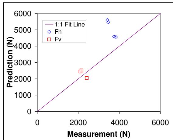
Figure 5: Comparison of model predictions with force measurements for IOT's tests dominated by shear failure: 60^\circ cone, 110 mm ice and ice velocity > or = 0.15\text{m/s} .
