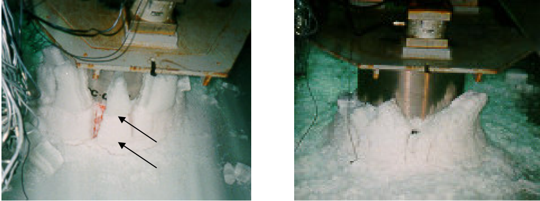
Figure 1. Photographs showing 110 mm thick ice interacting with a 60° cone at velocity 0.1m/s in the left picture (below the transitional speed) and at 0.25m/s in the right picture (above the transitional speed).
