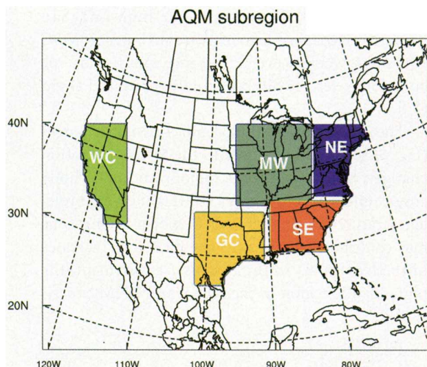
Fig. 6. The averaging subregions used in Fig. 7.
