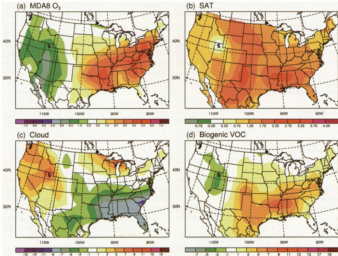
FIG. 9. As in Fig. 8 but for the CMU global modeling experiment (see Table 3).
