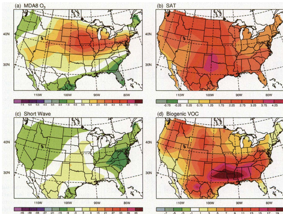
FIG. 8. Future-minus-present differences in simulated summertime mean (a) MDA8 O_3 concentration (ppb); (b) near-surface air temperature ( ^{\circ}C ); (c) surface insolation ( W m^{-2} ); and (d) biogenic isoprene emissions ( g C m^{-2} sec^{-1} ) for the Harvard I global modeling experiment (see Table 3).
