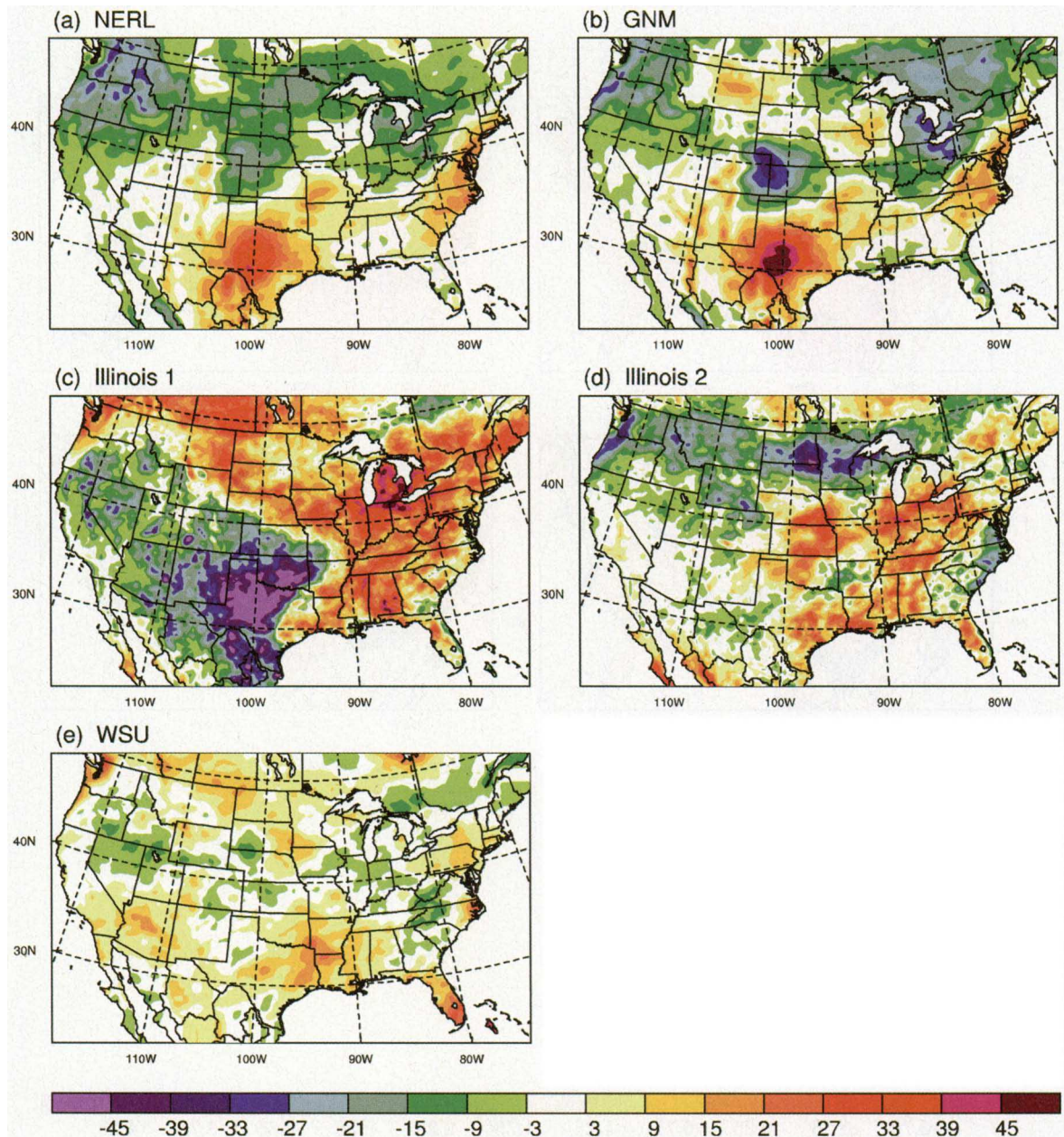
FIG. 4. As in Fig. 1, but for surface insolation ( \text{W m}^{-2} ).
