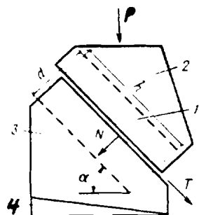
Figure 26. Schematic diagram of wedge apparatus
