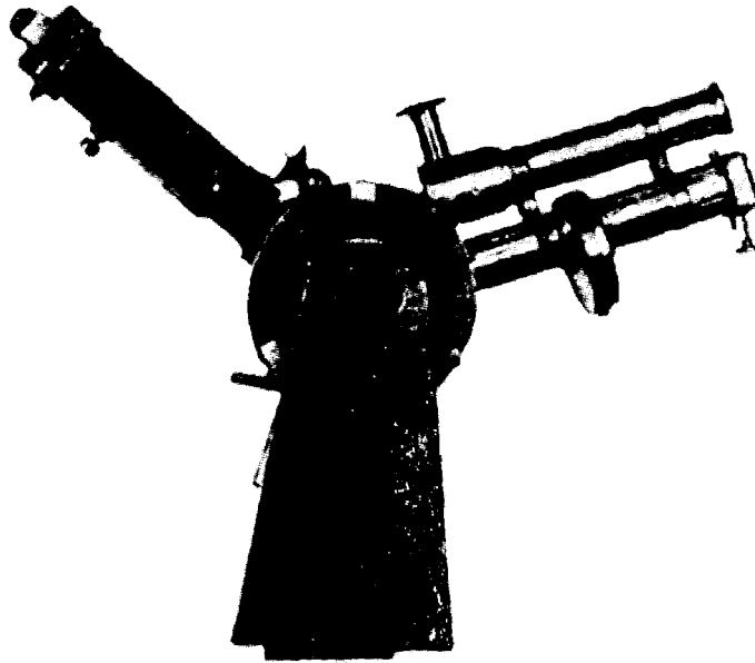
Fig. 1. N.I.L. Field Spectrograph.
