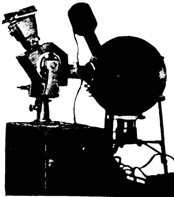
Fig. 6. Assembly of the Taylor sphere and spectrograph to measure the spectral reflectances.
