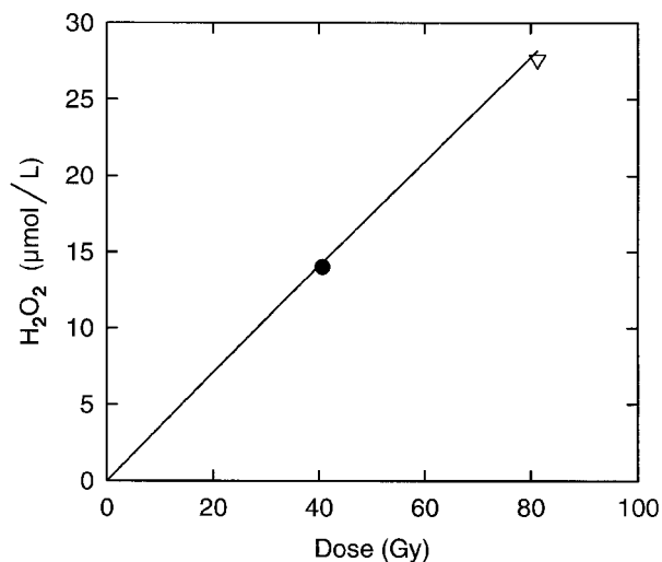
Fig. 2. The concentration of \text{H}_2\text{O}_2 versus dose, for \text{H}_2/\text{O}_2 water in the stirred water calorimeter under normal operating conditions. The ● represents two measurements and ▽ represents a single measurement (see Table 3). The solid line represents the computer simulation using model III.
