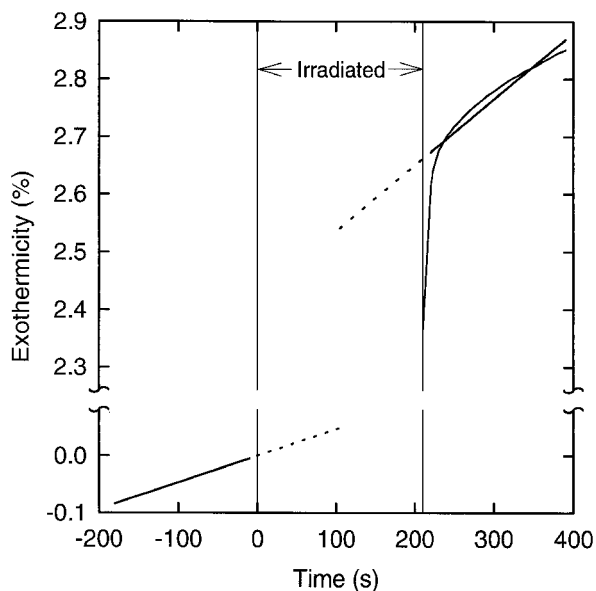
Fig. 1. Computer simulation of the temperature rise, presented as percent exothermicity, for \text{H}_2/\text{O}_2 water at a dose rate of 4.1 \text{ Gy min}^{-1} in the stirred water calorimeter. The simulation presented is for a single irradiation period mid-way through a set of 10 irradiation periods under the actual operating conditions of the calorimeter. Dose was delivered from 0 s to 210 s. The straight line before 0 s is the linear regression of the temperature rise between -180 s and -10 s and the percent exothermicity is set to zero at 0 s. The temperature rise before 0 s is due solely to the previous irradiations, i.e., for the first irradiation the exothermicity would be 0.0 % at all times up to the start of the irradiation. The curved line after 210 s represents the calculated percent exothermicity and the straight line between 220 s and 390 s is the linear regression of the curved line between 220 s and 390 s. The dashed lines are the extrapolations to mid-irradiation of the linear regressions.
