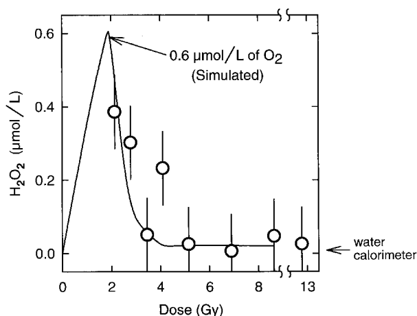
Fig. 5. Concentration of \text{H}_2\text{O}_2 versus dose for \text{H}_2 -saturated water containing a trace of \text{O}_2 and irradiated in a vessel with no gas space. The data points represent experimental measurements for solutions containing (5 \pm 1) \times 10^{-7}\text{ mol L}^{-1} of \text{O}_2 . The solid line represents a simulation for 6 \times 10^{-7}\text{ mol L}^{-1} of \text{O}_2 . The arrow outside the graph indicates the average measured value for \text{H}_2 -saturated water irradiated to doses of about 13 Gy in our water calorimeter under standard operating conditions.
