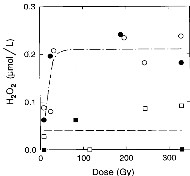
Fig. 4. The concentration of \text{H}_2\text{O}_2 for pure and \text{H}_2 -saturated water as a function of dose. Pure water at 21\text{ }^\circ\text{C} is indicated by \circ and at 0\text{ }^\circ\text{C} is indicated by \bullet ; the dash-dot line is only an aid to the eye. \text{H}_2 -saturated water at 21\text{ }^\circ\text{C} is indicated by \square and at 0\text{ }^\circ\text{C} is indicated by \blacksquare ; the dashed line is only an aid to the eye.
