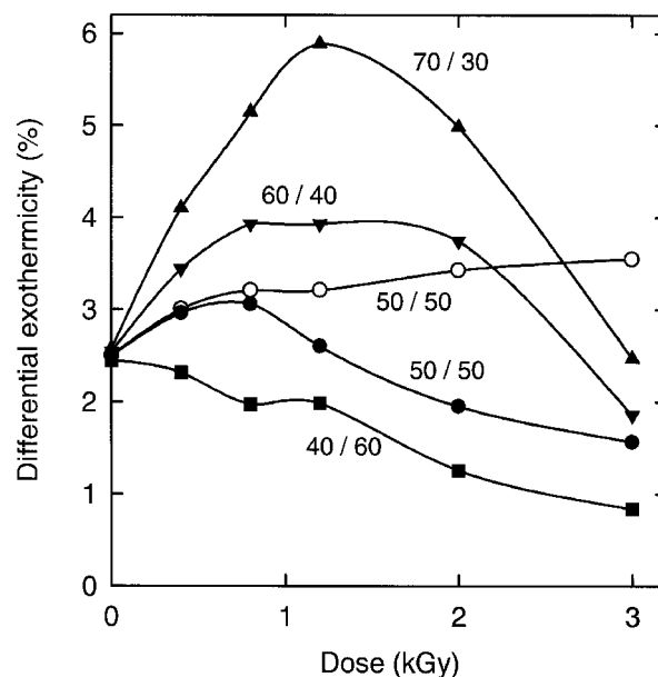
Fig. 3. Simulations of the differential percent exothermicity for water, equilibrated with various mixtures of \text{H}_2 and \text{O}_2 before irradiation and irradiated in the absence of a gas space. X/Y indicates that the gas mixture used to saturate the water was made up of an amount-of-substance fraction of \text{H}_2 = X % and an amount-of-substance fraction of \text{O}_2 = Y %. Hence, the ratio 50/50 designates the same solution referred to in this report as \text{H}_2/\text{O}_2 water. Only for the simulation denoted by \circ , were the concentrations of \text{H}_2 and \text{O}_2 in the solution forced to remain constant throughout the simulation. Otherwise, the simulations allowed the concentrations of \text{H}_2 and \text{O}_2 to change as dictated by the radiolysis. The differential values of the percent exothermicity were calculated for a dose of 3.1 Gy which took the accumulated dose to the dose indicated for the data point.
