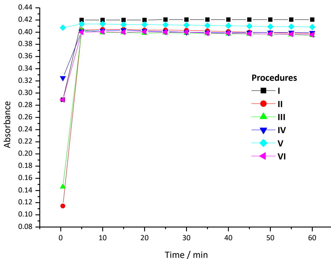
Figure 3. Effect of time on development of the [CrDPCO] + complex. Different procedural media spiked with 0.5 \mu\text{g mL}^{-1} Cr(VI).
