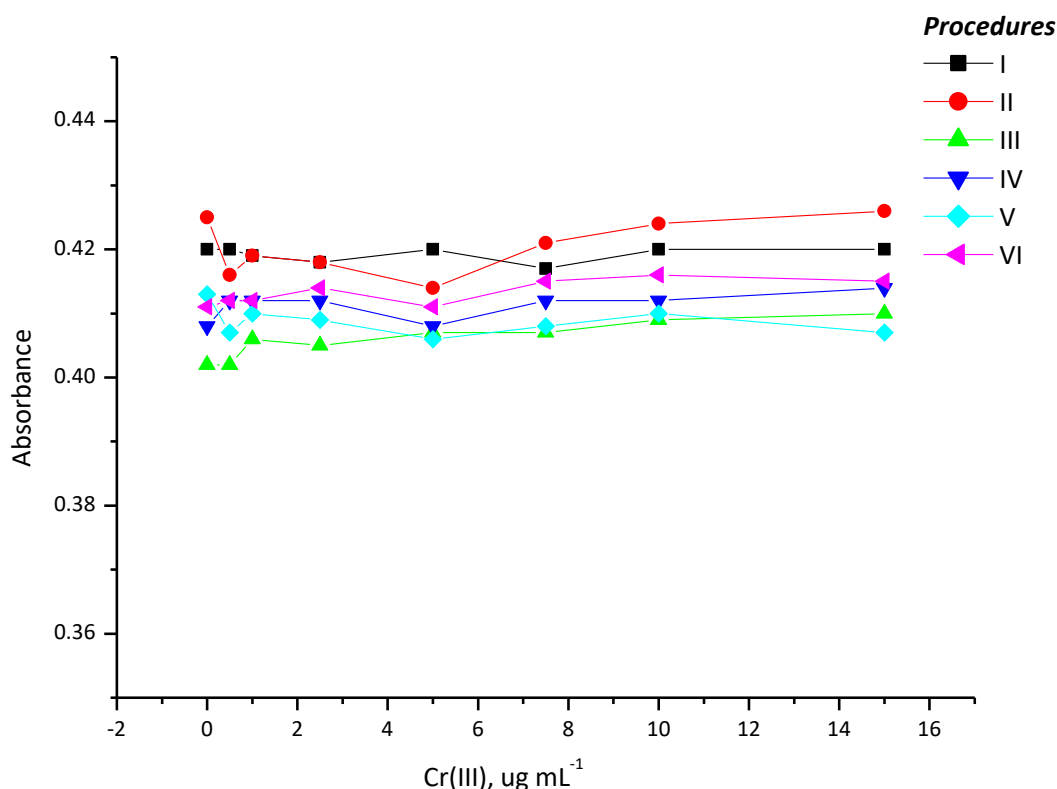
Figure 4. Effect of added Cr(III) in different extraction media. Standard of 0.5 µg mL -1 Cr(VI) spiked with varying concentrations of Cr(III) and subjected to extraction procedures I to VI.
