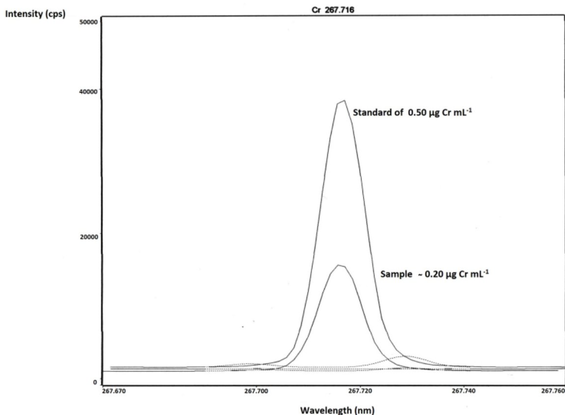
Figure 1. Emission spectra generated by introduction of a sample solution prepared using Procedure (II) and a 0.50 \mu\text{g Cr mL}^{-1} calibration standard. Dotted lines reflect procedural blanks; that with a peak at 267.73 nm arises from a processed sample.
