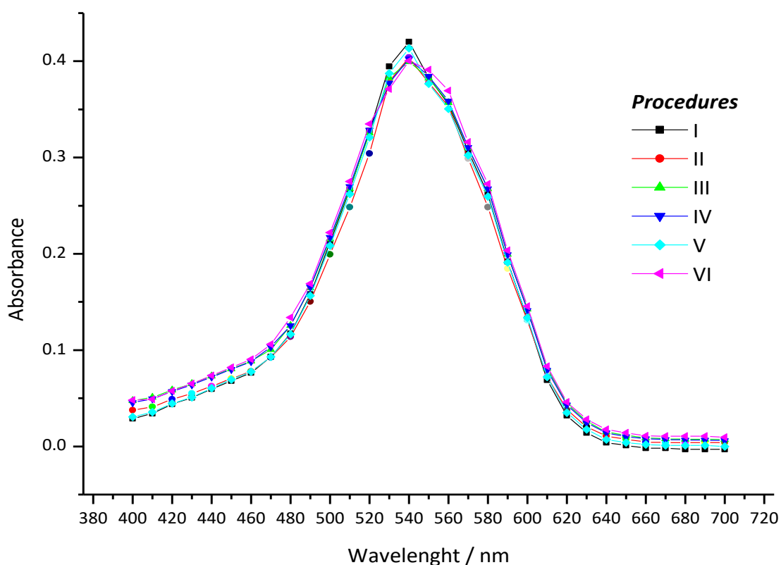
Figure 2. Effect of various Cr 2 O 3 pigment extraction media on absorbance band structure. Each solution was spiked with 0.5 \mu\text{g mL}^{-1} Cr(VI).
