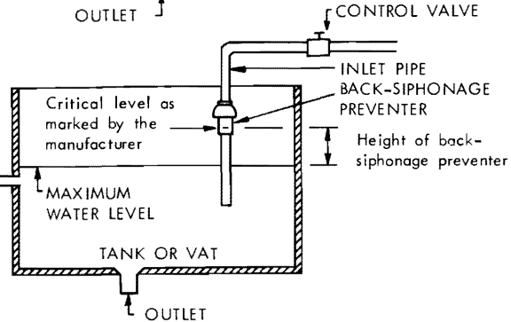
(b) In tank or vat
