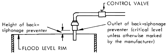
(a) Above flood level rim
