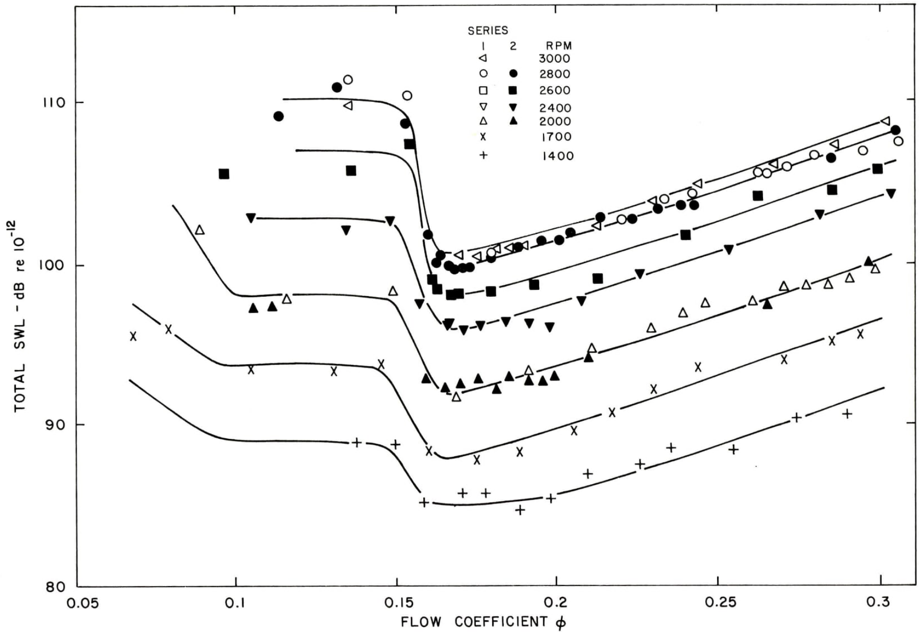
FIG. 10: TOTAL SWL AGAINST FLOW COEFFICIENT 0.4437 m DIAMETER FAN, n_s = 1.466 SET
