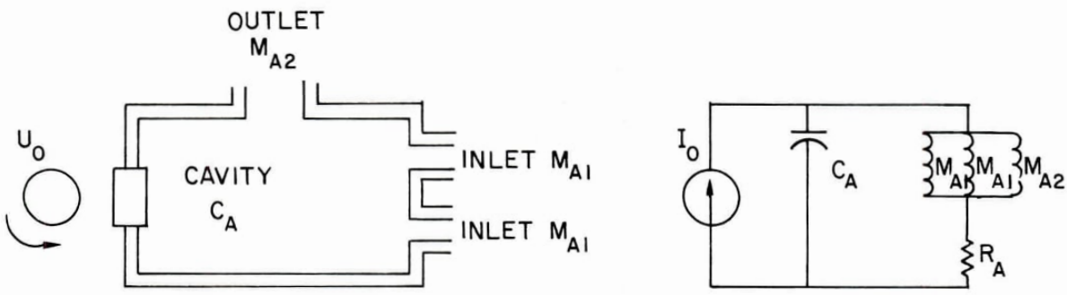
DOUBLE INLET
