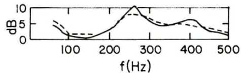
FIG. 27: RESULTS OF MEASUREMENTS ON A FULL-SCALE AXIAL FAN, USING THE ONE PORT FAN SYSTEM TEST RIG (REF. 12)
