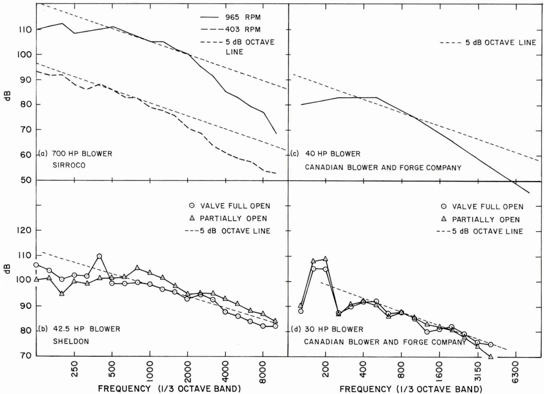
FIG. 35: NOISE SPECTRA FROM LARGE BLOWERS
