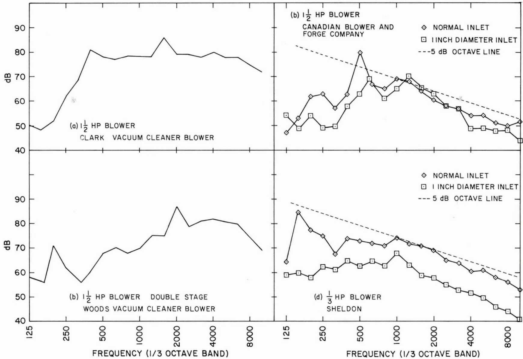
FIG. 37: NOISE SPECTRA FROM SMALL BLOWERS
