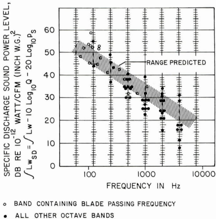
FIG. 8: MEASURED SOUND POWER LEVELS OF A GROUP OF EIGHT FANS WITH BACKWARD CURVED BLADES WITH PREDICTED RANGE (REF. 5)
