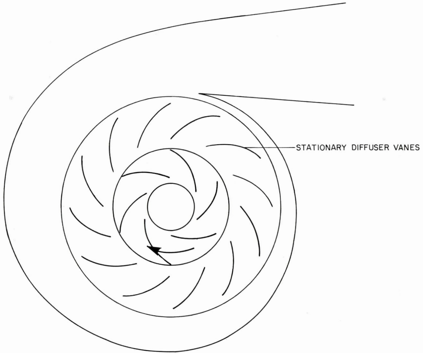
FIG. 3: VOLUTE WITH VANED DIFFUSER
