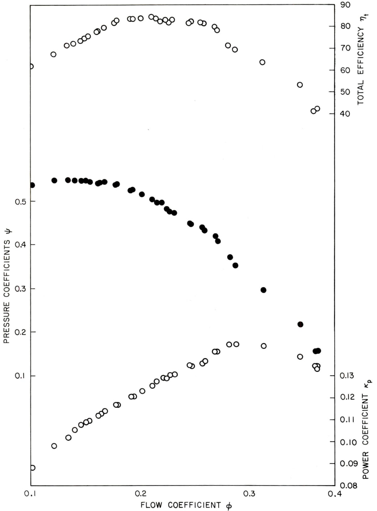
FIG. 11: CHARACTERISTIC OF 1.1552 m DIAMETER FAN AT 750 rev./min., n_s = 0.822 SET (REF. 9)
