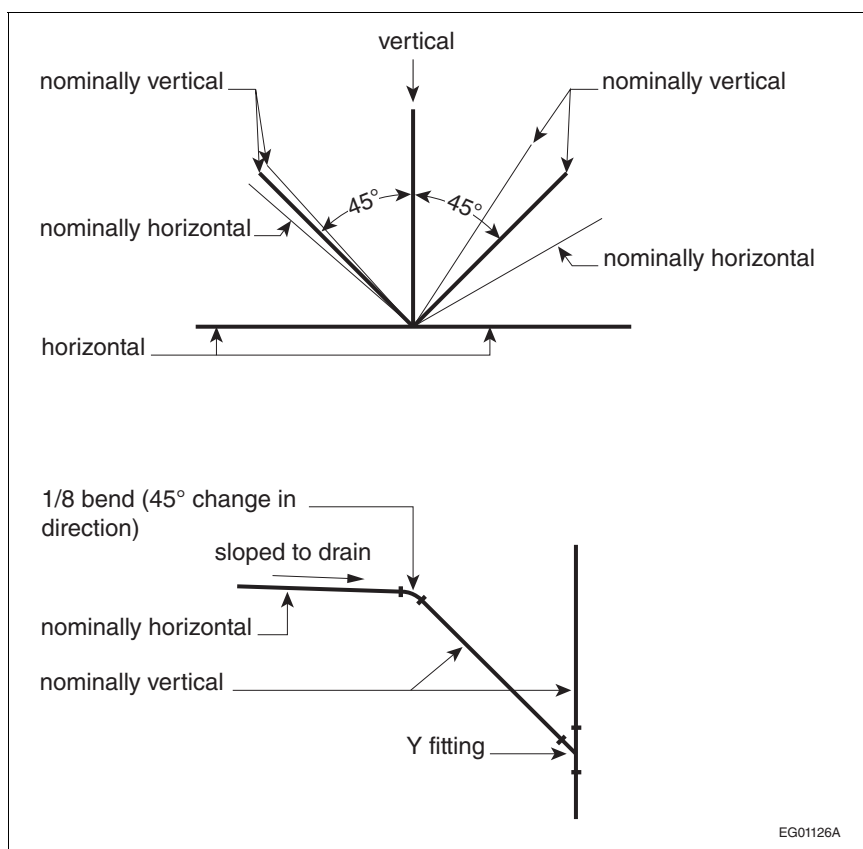
Figure A-1.4.1.2.(1)-J Nominally horizontal and nominally vertical
