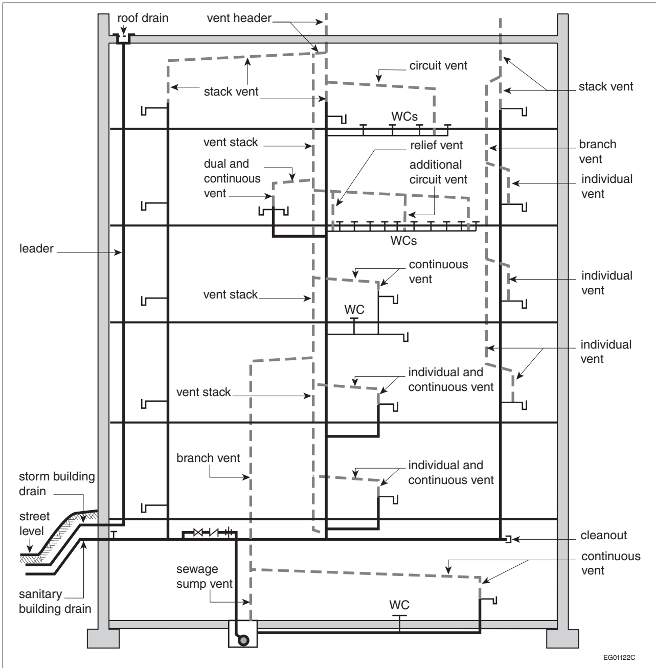
Figure A-1.4.1.2.(1)-G Venting system
