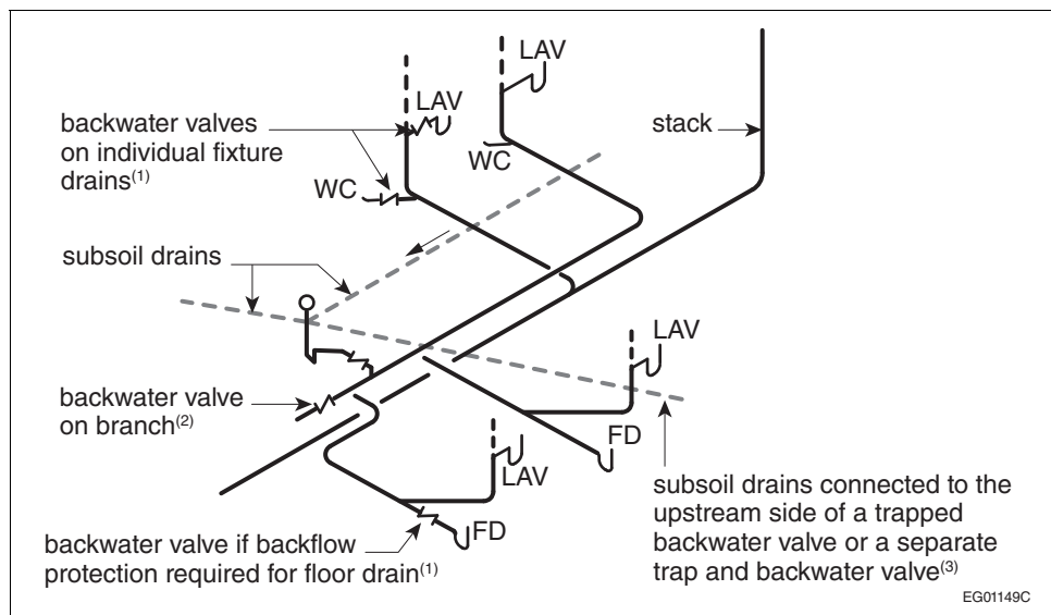
Figure A-2.4.6.4.(1) Protection from backflow caused by surge
