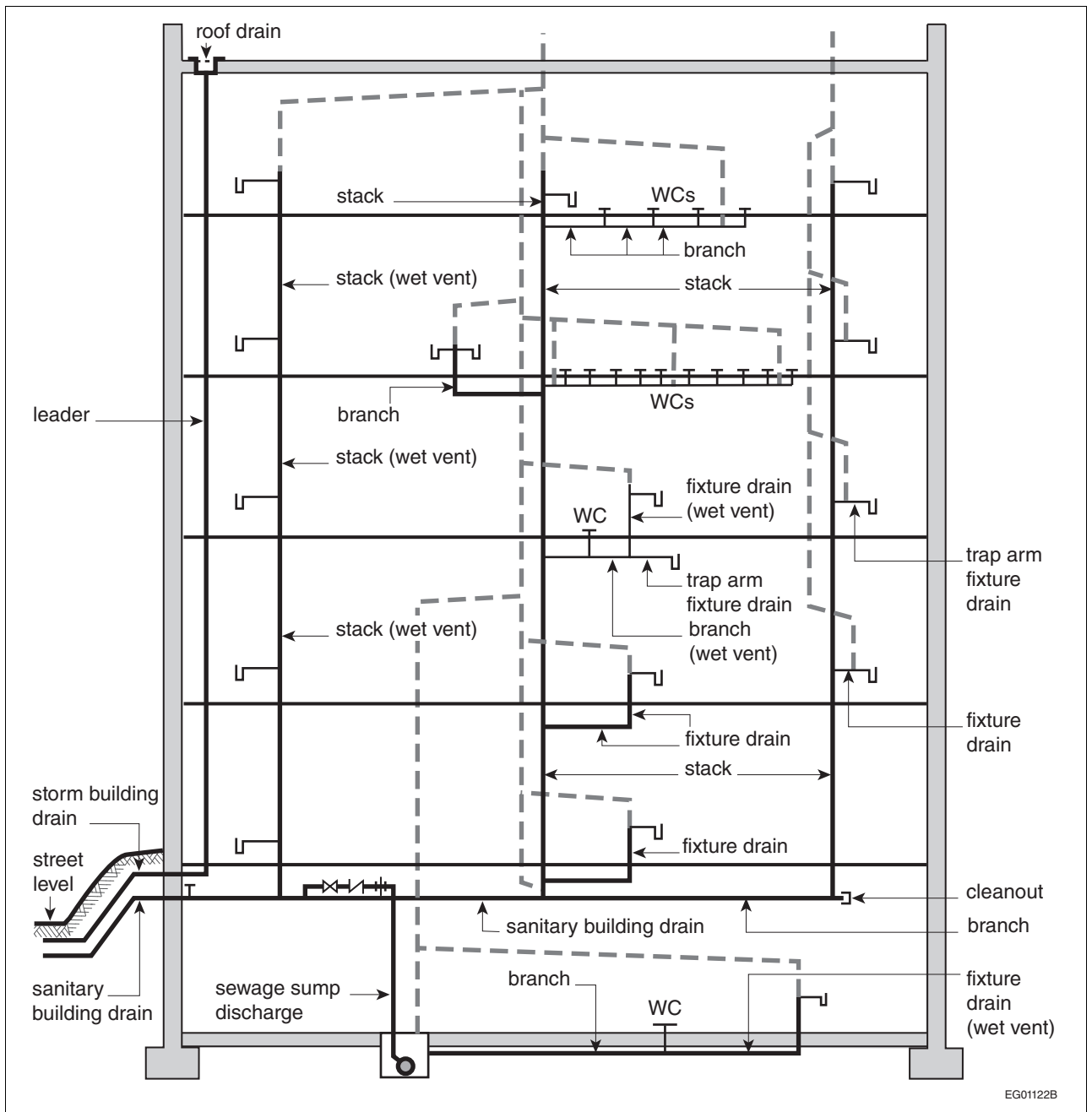
Figure A-1.4.1.2.(1)-F Drainage system
