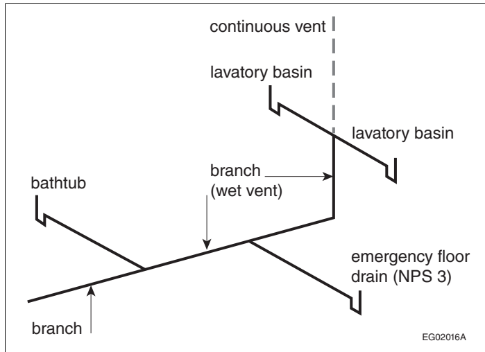
Figure A-2.5.2.1-D Example of wet venting described in Clause 2.5.2.1.(1)(e)
