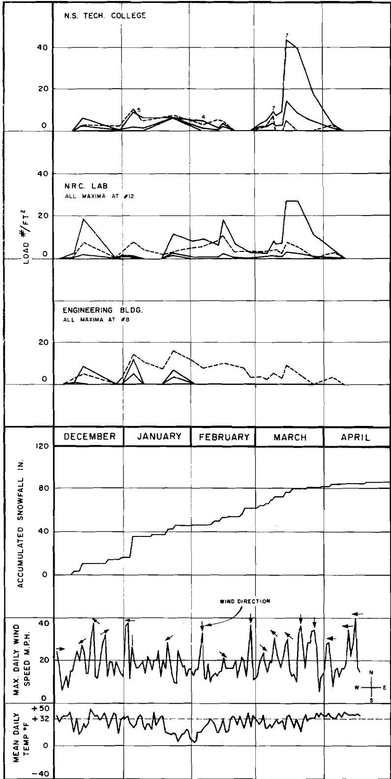
SNOW LOAD OBSERVATIONS ON ROOFS
