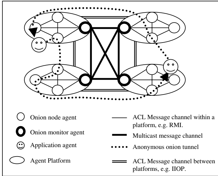
Figure 1. Agent-based Onion Routing Topology
