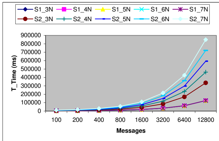
Figure 8. T_Time for the model 2
