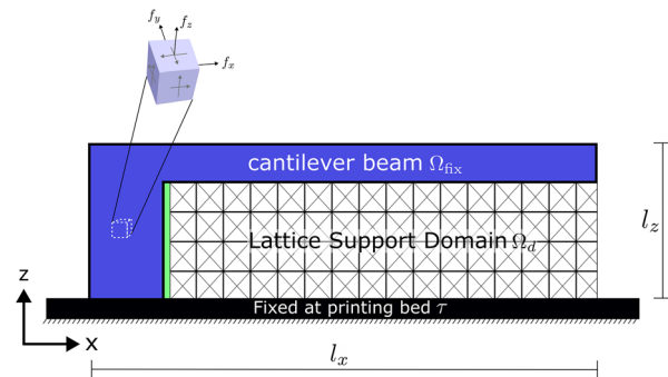
Figure 1. Design domain of lattice support structure for cantilever beam. Both cantilever beam ( \Omega_{fix} ) and lattice support ( \Omega_d ) restrained at printing bed \tau ; and \Omega_{fix} subjected to body force f_{xyz} .
