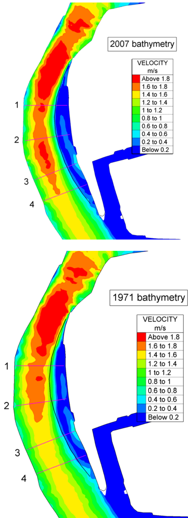
Figure 16 - Recirculation zone in first bend of St.Clair River
