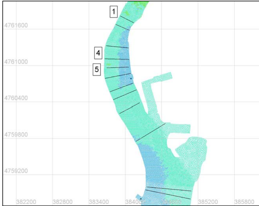
Figure 5 - Cross-section location
