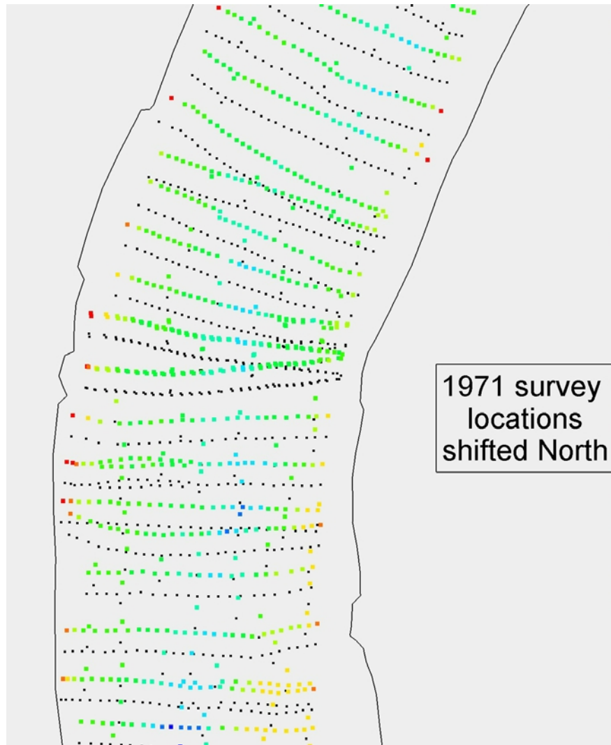
Figure 22 - Bend upstream of Fawn Islands shifted North
