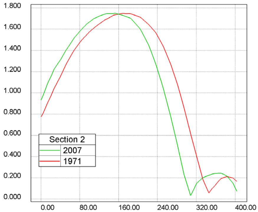
Figure 17 - Transverse section of water velocity profile (m/s), in sections 1 and 2
