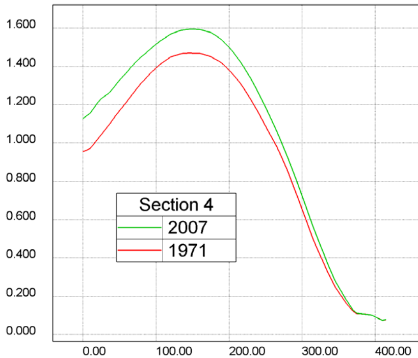
Figure 18 - Transverse section of water velocity profile (m/s), in sections 3 and 4
