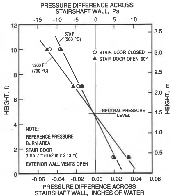
Figure 6 Pressure difference across stairshaft wall with stair door open and closed on fire floor
