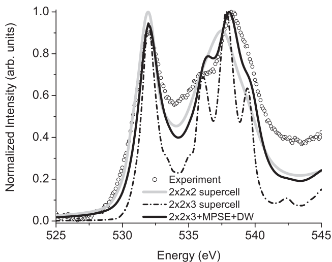
FIG. 3. Oxygen- K -edge spectra from \text{SnO}_2 . Experimental: open circles; calculated using WIEN2K for supercells of different sizes. The black solid line corresponds to a 2 \times 2 \times 3 spectrum convolved to account for the self-energy.
