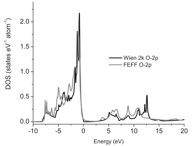
FIG. 4. Oxygen p DOS obtained from calculations using FEFF (gray line) and WIEN2K (black line). The zero of energy is the Fermi level.
