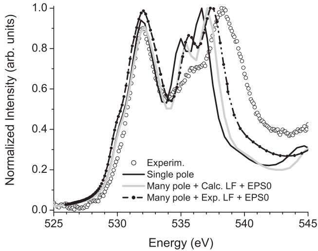
FIG. 2. Oxygen- K -edge spectra from \text{SnO}_2 . Experimental: open circles; calculated using FEFF: single pole (black solid line), many poles with a calculated loss function and EPS0 (light gray), and many poles with an experimental loss function and EPS0 (black dashed-dot line).
