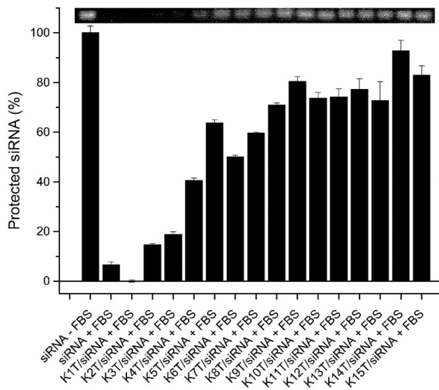
Fig. 5 Protective ability of siRNA by Knt RNTs ( n = 1-15 ) in presence of FBS (+FBS) compared to the control of siRNA without FBS (-FBS).
