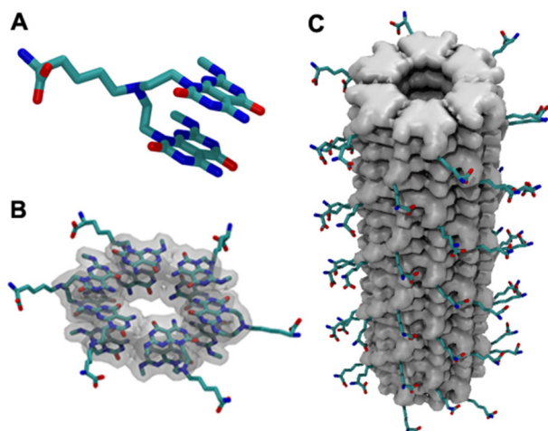
Fig. 2 Lysine functionalized twin-G \wedge C motif K1T (A). Hierarchical self-assembly of K1T into double-stacked hexameric rosettes (B) which then further \pi - \pi stack to form RNTs (C).
